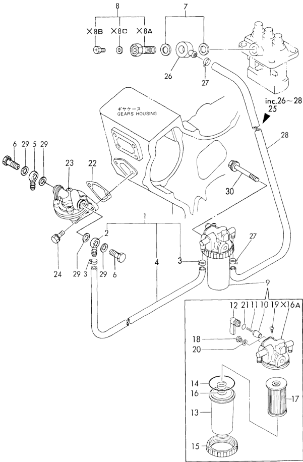
Fig.12. FUEL LINE
