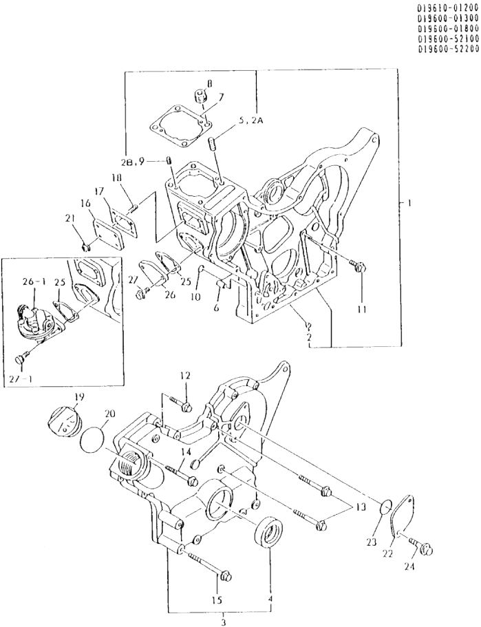
Fig.5. GEAR HOUSING
