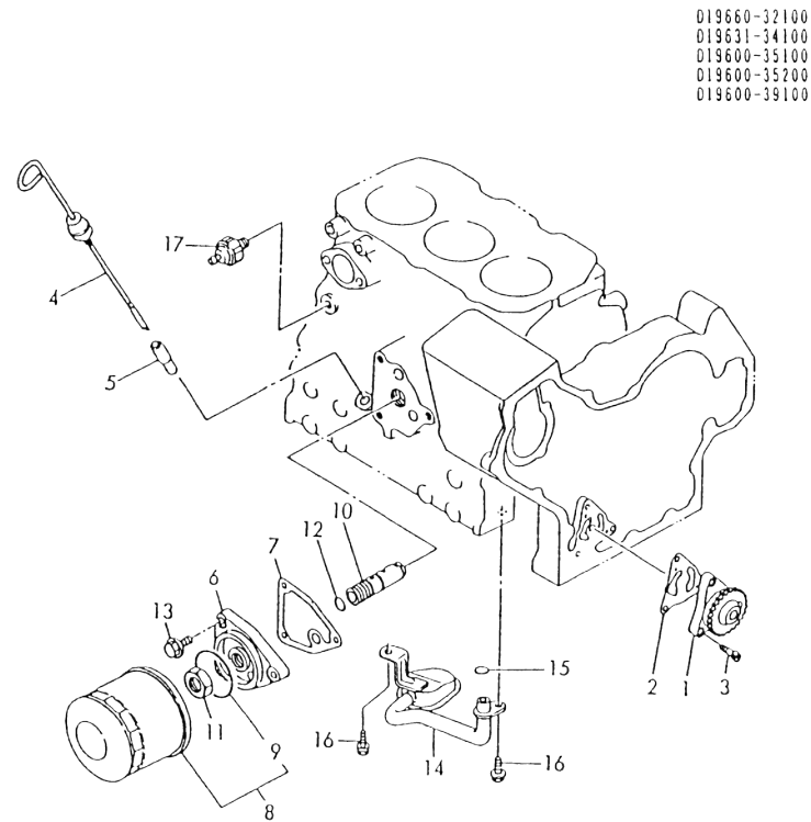
Fig.9. LUB.OIL SYSTEM
