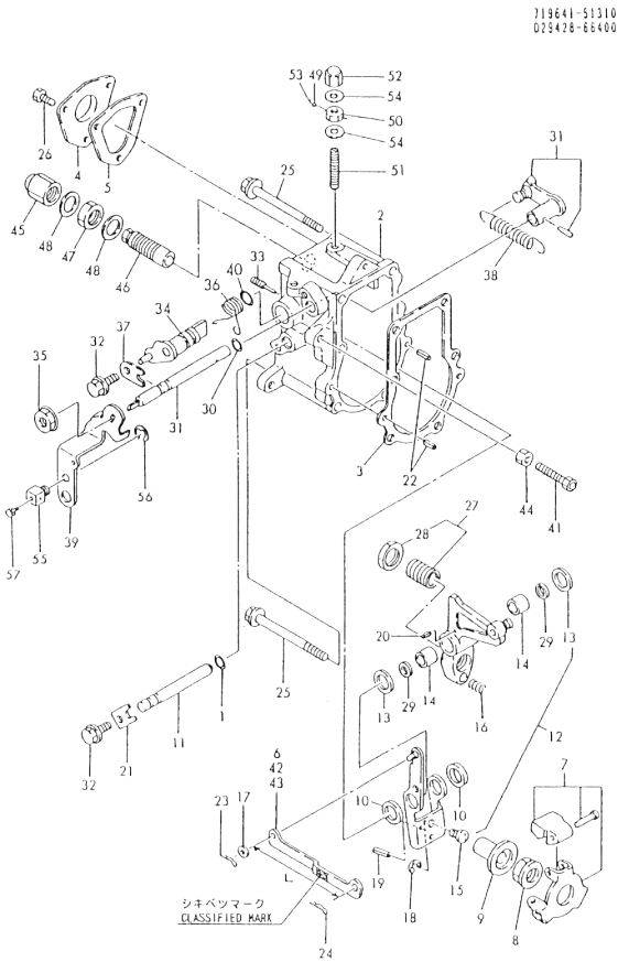
Fig.13. GOVERNOR
