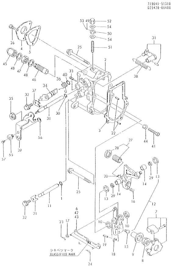
Fig.13. GOVERNOR
