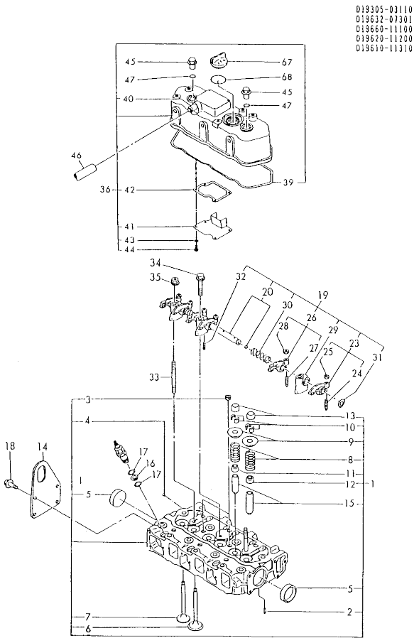
Fig.4. CYLINDER HEAD & BONNET
