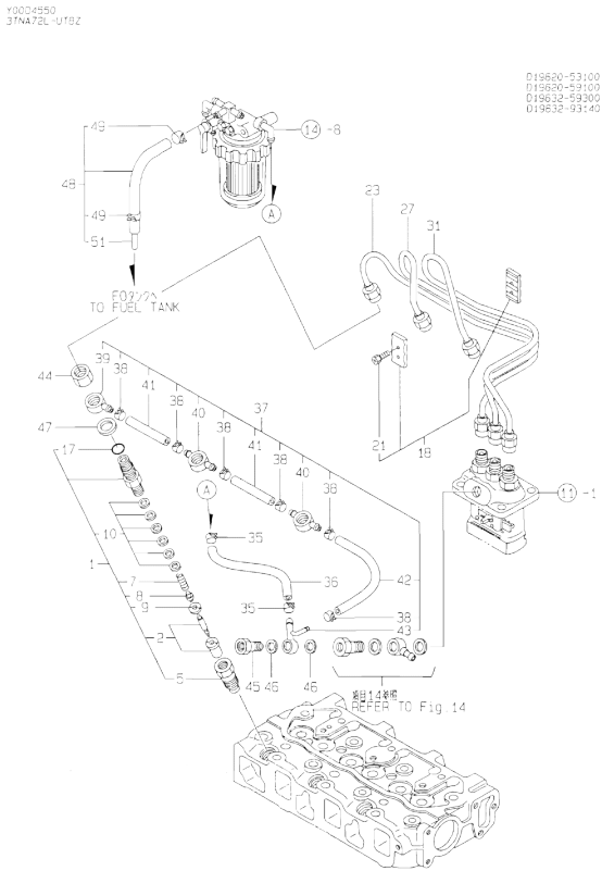
OCD10-M45500 3TNA72L-UTBZ Fig.13. FUEL INJECTION VALVE
