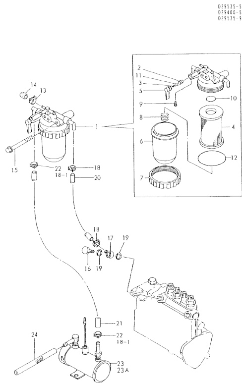
Fig.20. FUEL OIL SYSTEM
