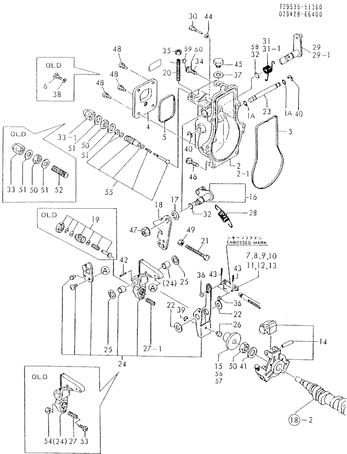
Fig.22. GOVERNOR
