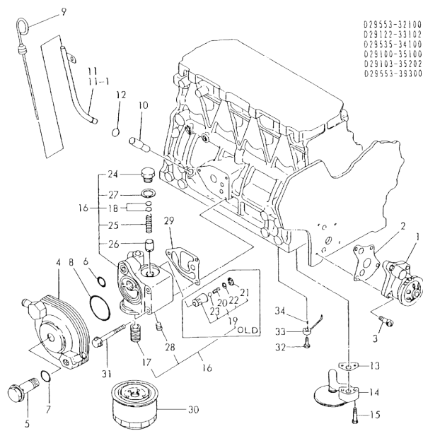
Fig.13. LUB. OIL SYSTEM
