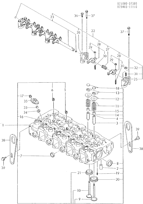
Fig.6. CYLINDER HEAD
