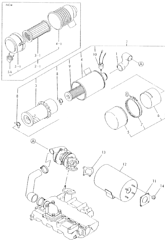
Fig.7. AIR CLEANER & SILENCER
