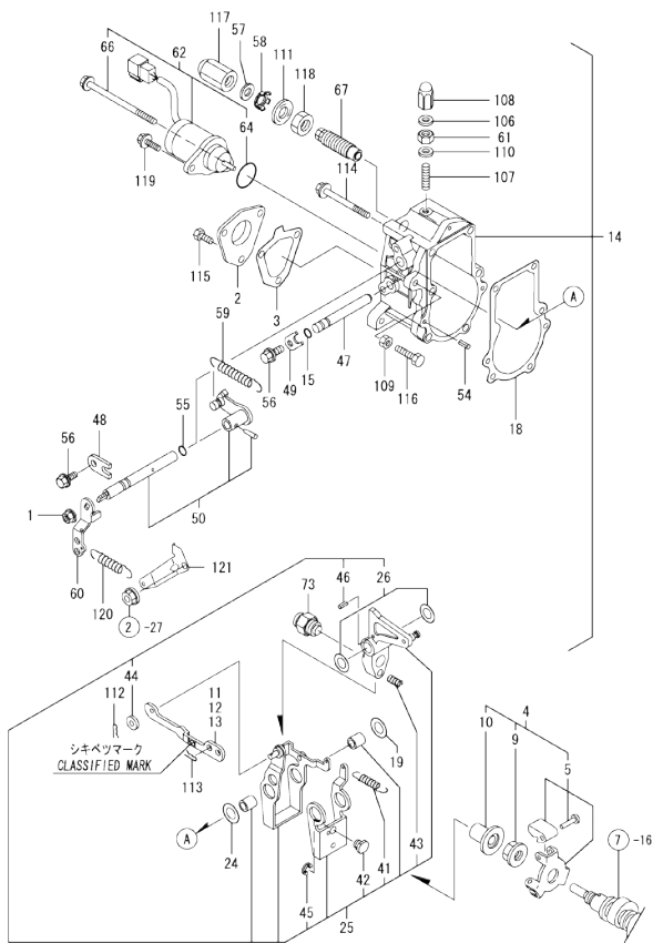
Fig.12. GOVERNOR
