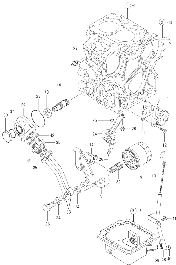
Fig.9. LUB.OIL SYSTEM
