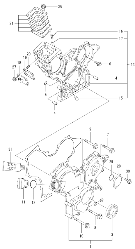
Fig.2. GEAR HOUSING
