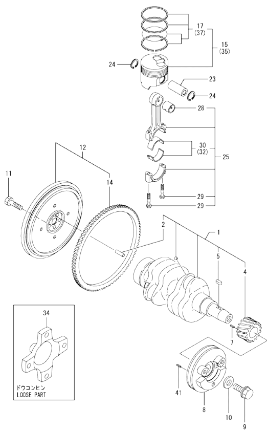
Fig.8. CRANKSHAFT & PISTON
