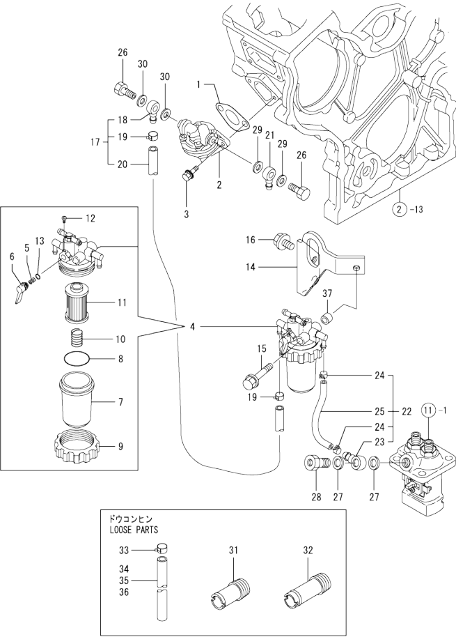
Fig.14. FUEL LINE
