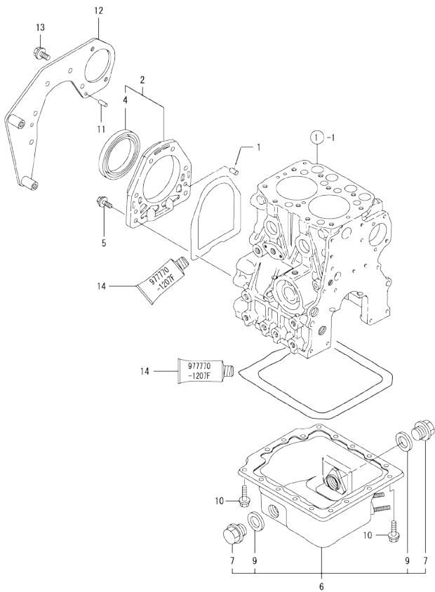
Fig.3. OIL SUMP
