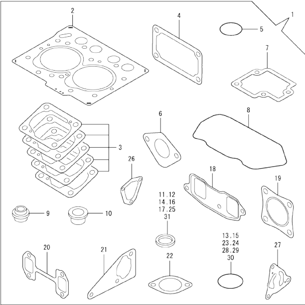
Fig.17. GASKET SET & TOOLS
