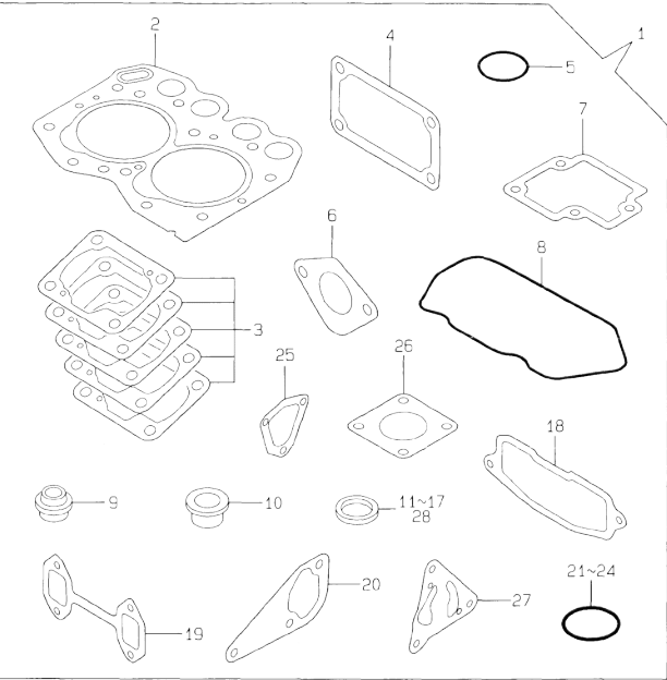
Fig.17. GASKET SET
