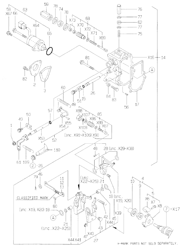
Fig.13. GOVERNOR
