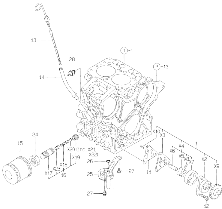
Fig.9. LUB.OIL SYSTEM
