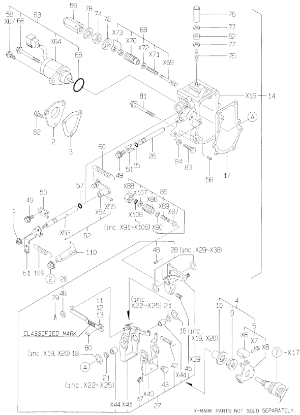
Fig.13. GOVERNOR
