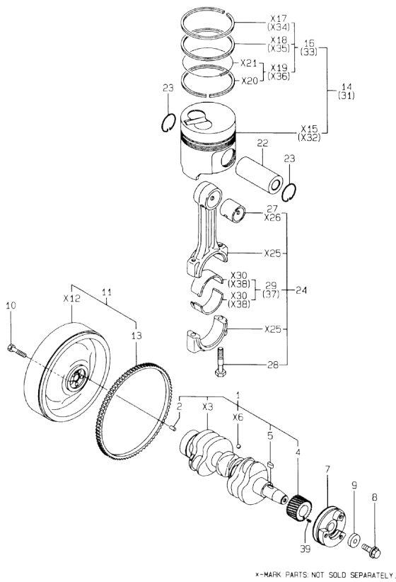
Fig.8. CRANKSHAFT & PISTON
