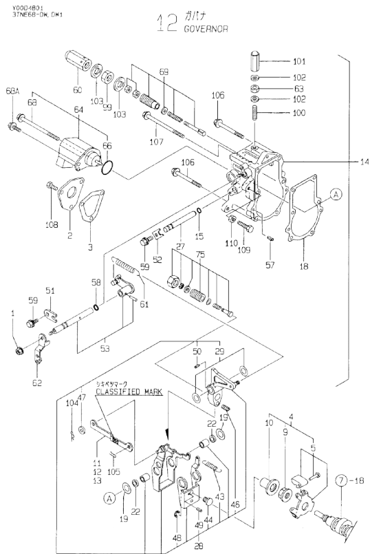
Fig.12. GOVERNOR
