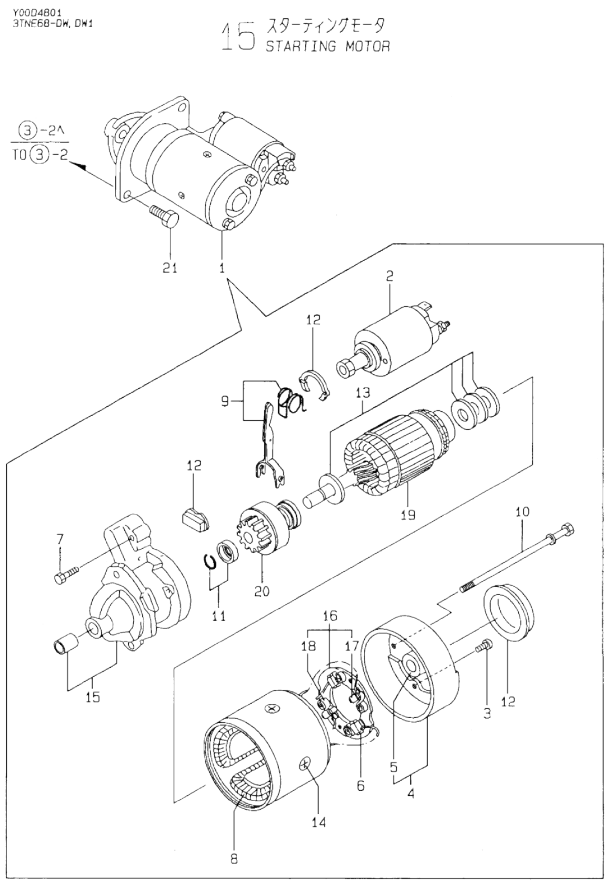
Fig.15. STARTING MOTOR
