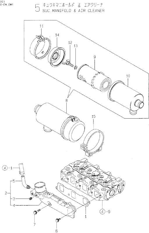
Fig.5. SUC.MANIFOLD & CLEANER
