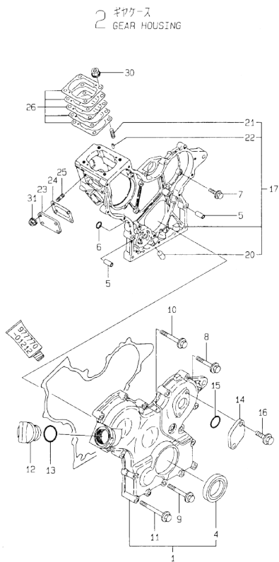
Fig.2. GEAR HOUSING
