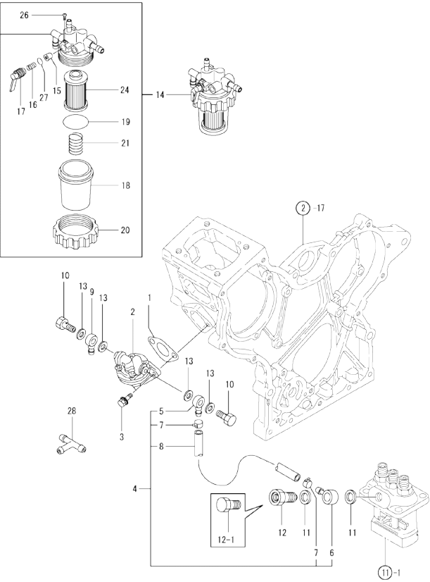
Fig.14. FUEL LINE
