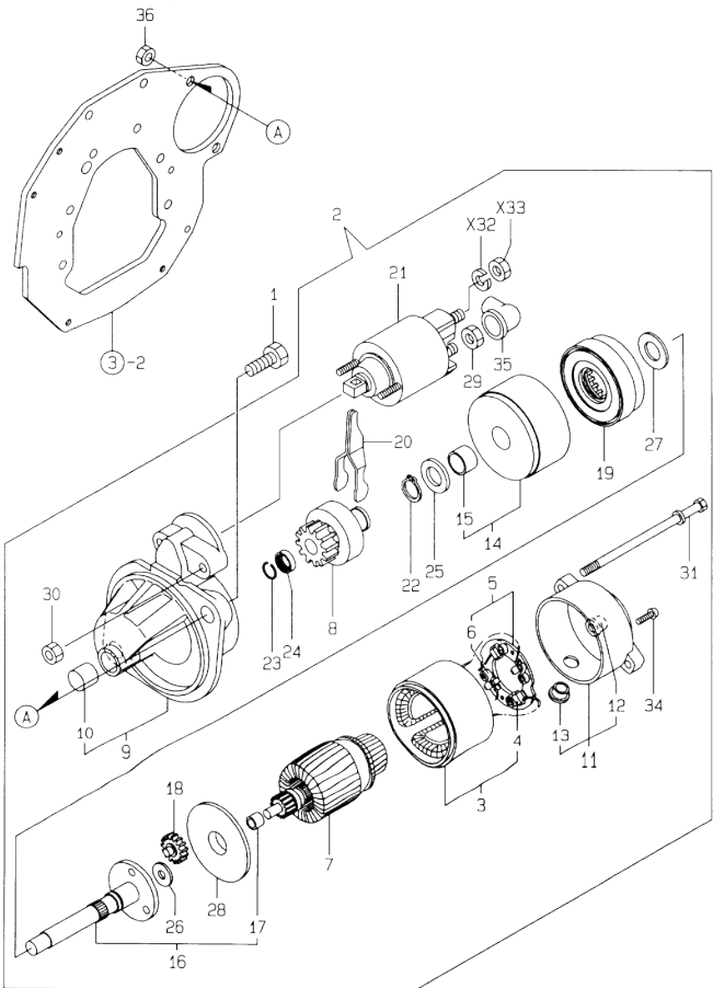
Fig.15. STARTING MOTOR
