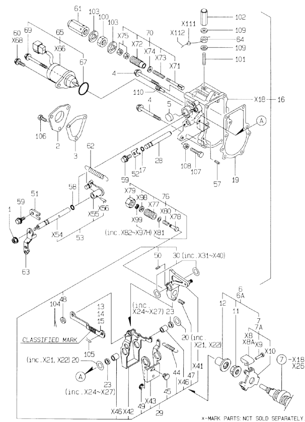
Fig.12. GOVERNOR
