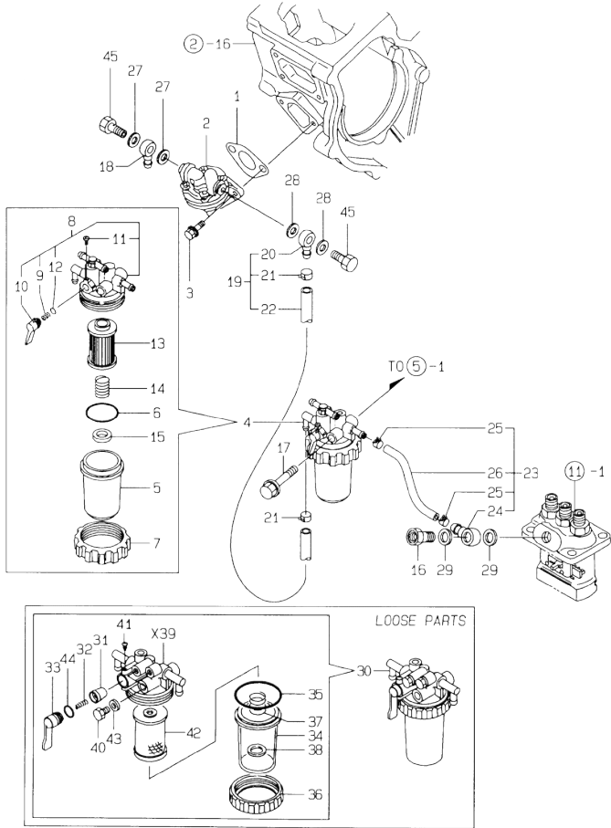
Fig.14. FUEL LINE
