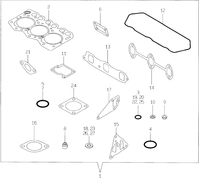
Fig.17. GASKET SET
