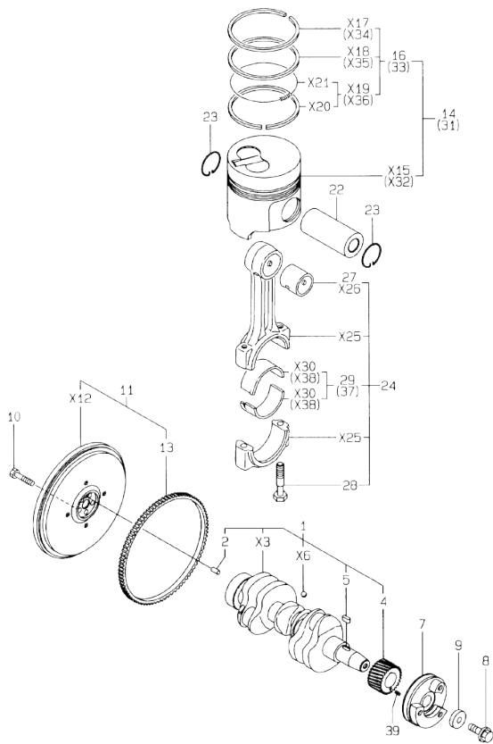
B. CRANKSHAFT & PISTON
