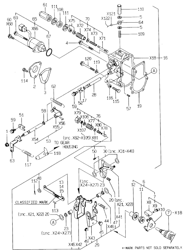
Fig.12. GOVERNOR
