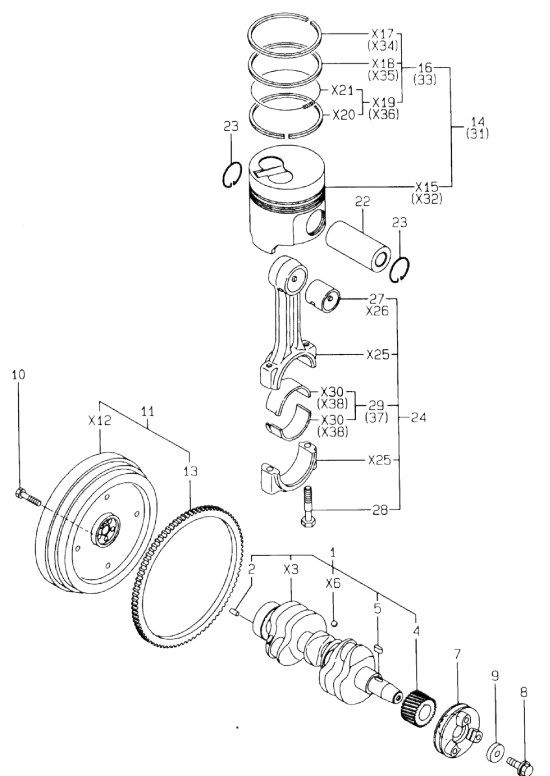
Fig.8. CRANKSHAFT & PISTON
