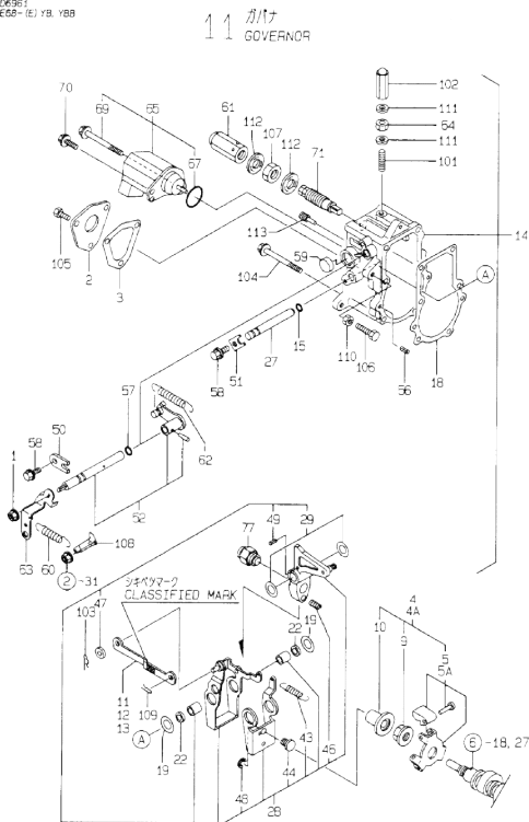
Fig.11. GOVERNOR
