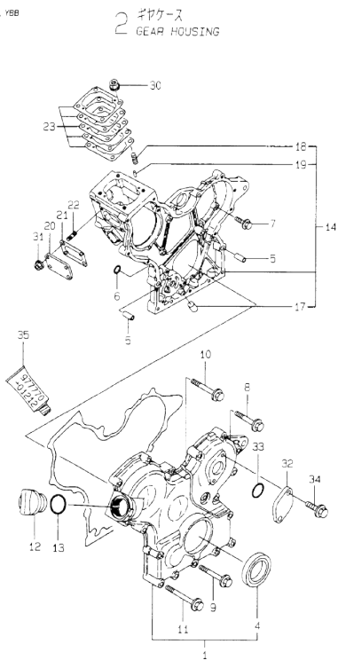
OCD10-M69601 3TNE68-(E)YB(B) Fig.2. GEAR HOUSING
