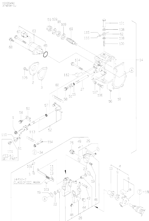
OCD10-M54900 3TNE68-SJ Fig.12. GOVERNOR
