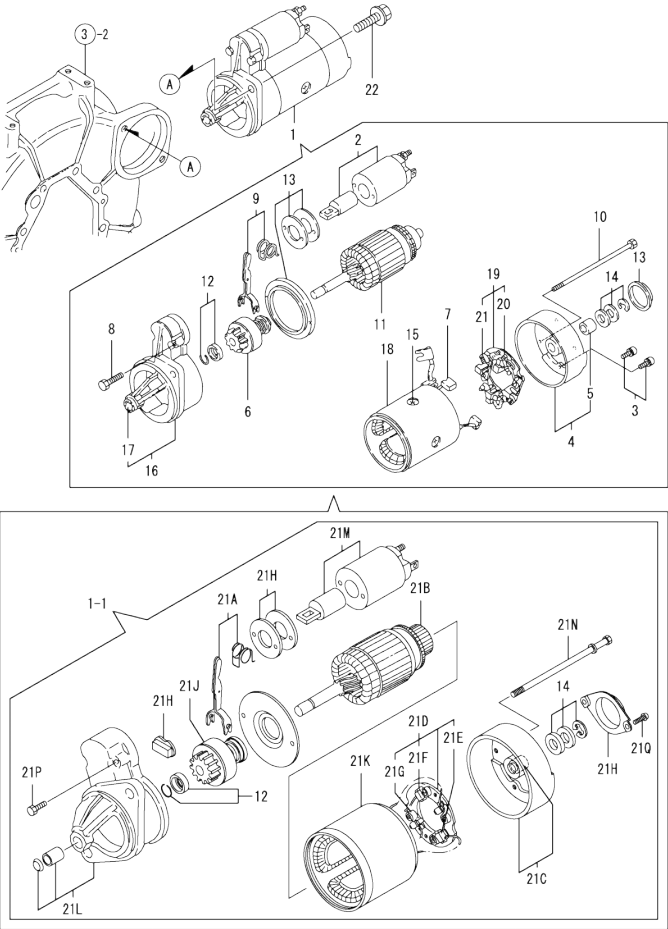
Fig.15. STARTING MOTOR
