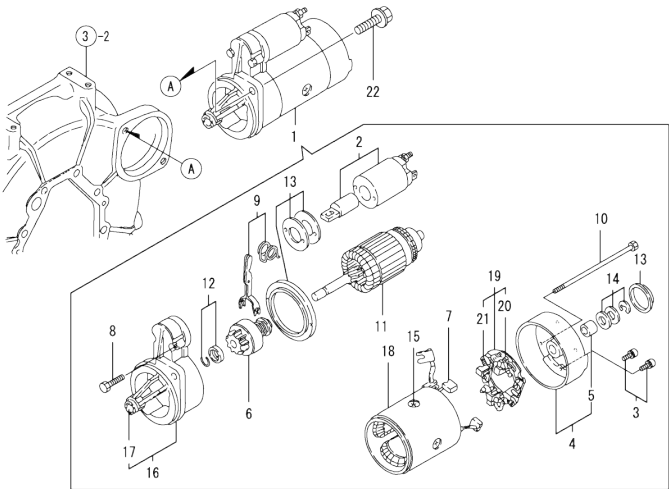
Fig.15. STARTING MOTOR
