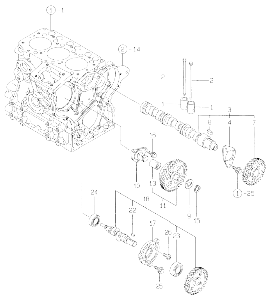
Fig.7. CAMSHAFT & DRIVING GEAR
