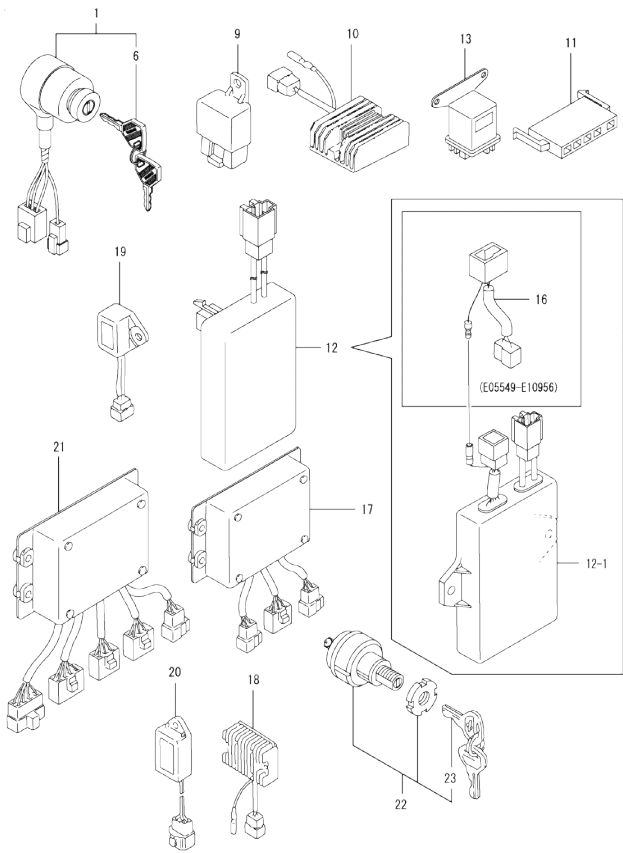
Fig.17. ELECTRIC PARTS
