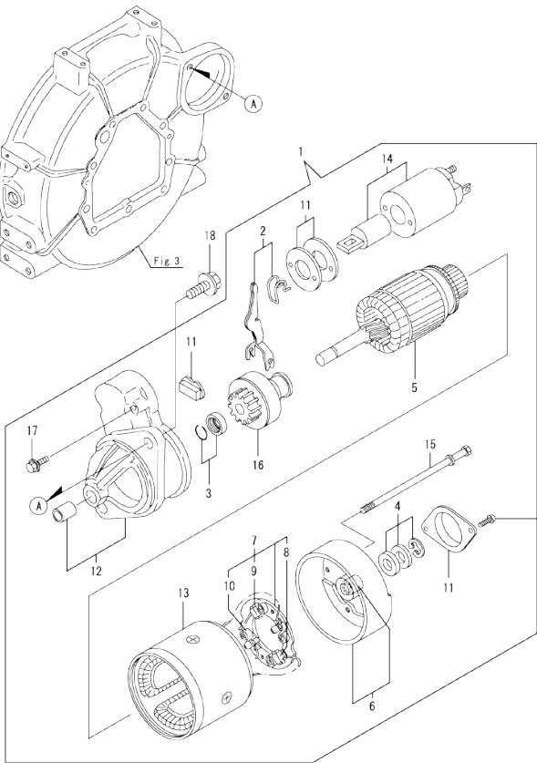
Fig.21. STARTER MOTOR
