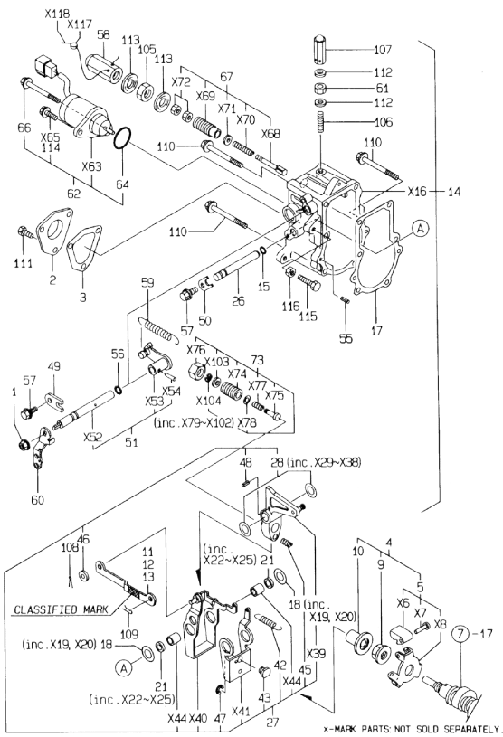
Fig.12. GOVERNOR
