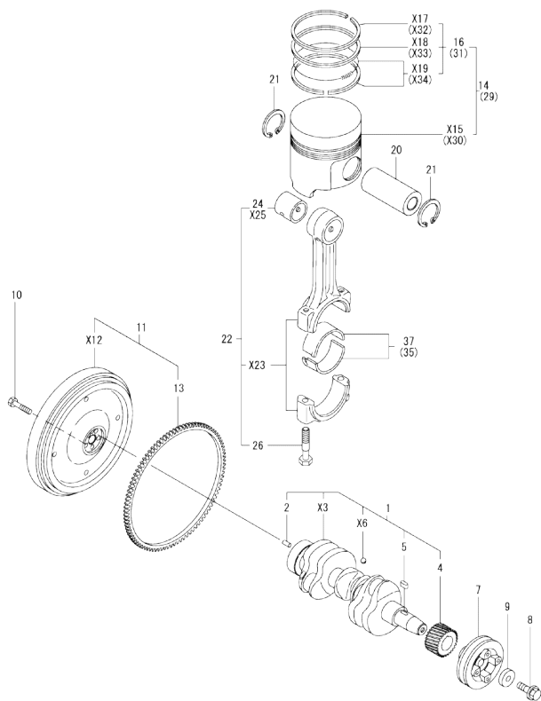
Fig.8. CRANKSHAFT & PISTON
