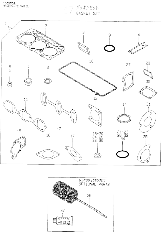
Fig.17. GASKET SET
