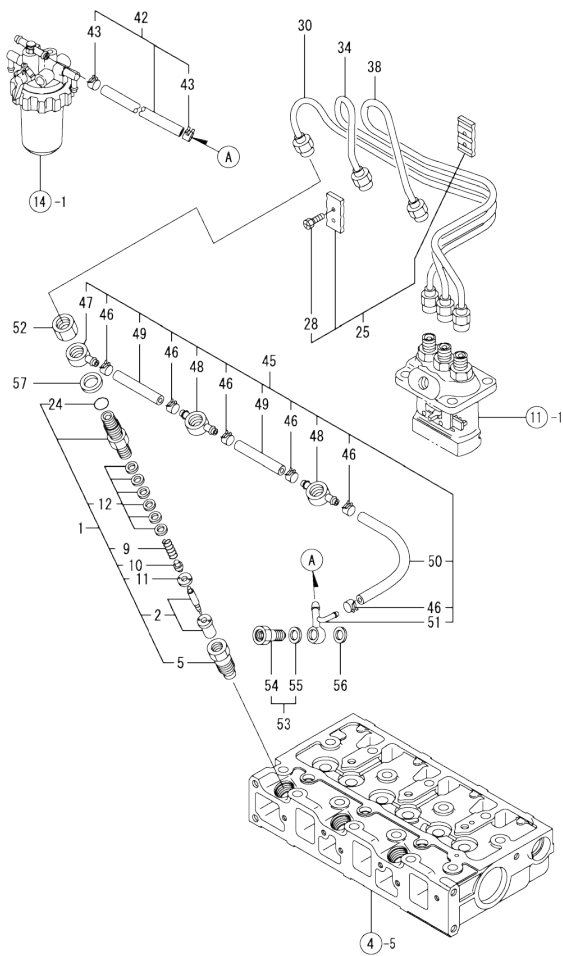
Fig.13. FUEL INJECTION VALVE
