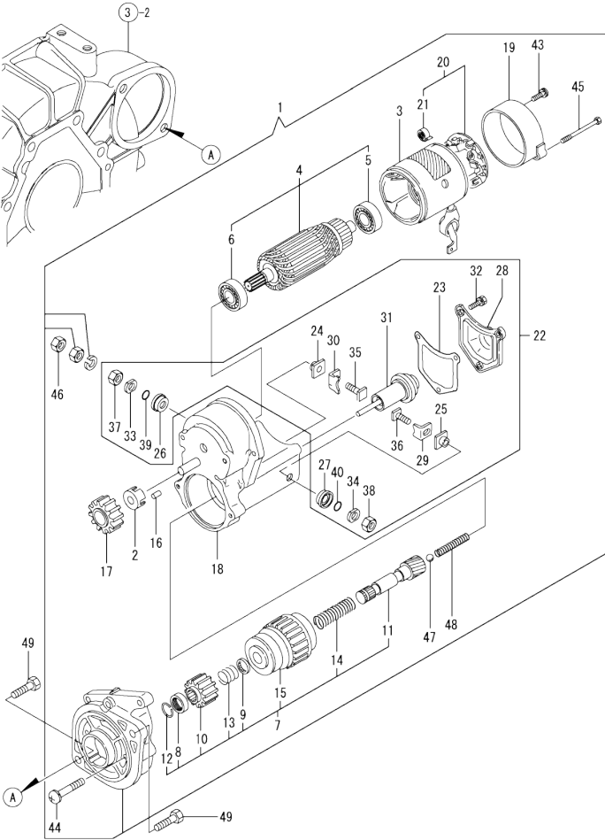
Fig.15. STARTING MOTOR
