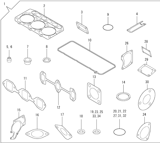
Fig.17. GASKET SET
