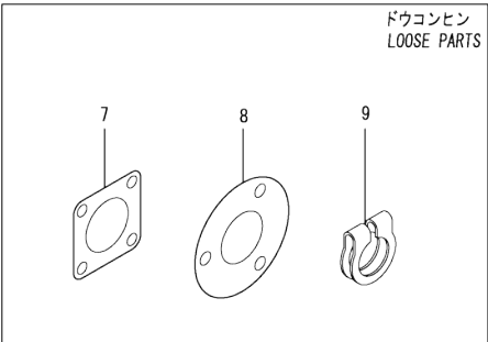
0CD10-M77700 ENGINE 3TNE74-ENYBC Fig.6. EXHAUST MANIFOLD
