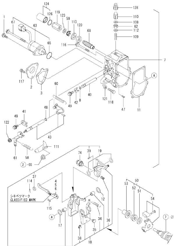
Fig.12. GOVERNOR
