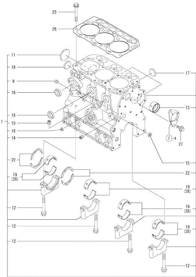
Fig.1. CYLINDER BLOCK
