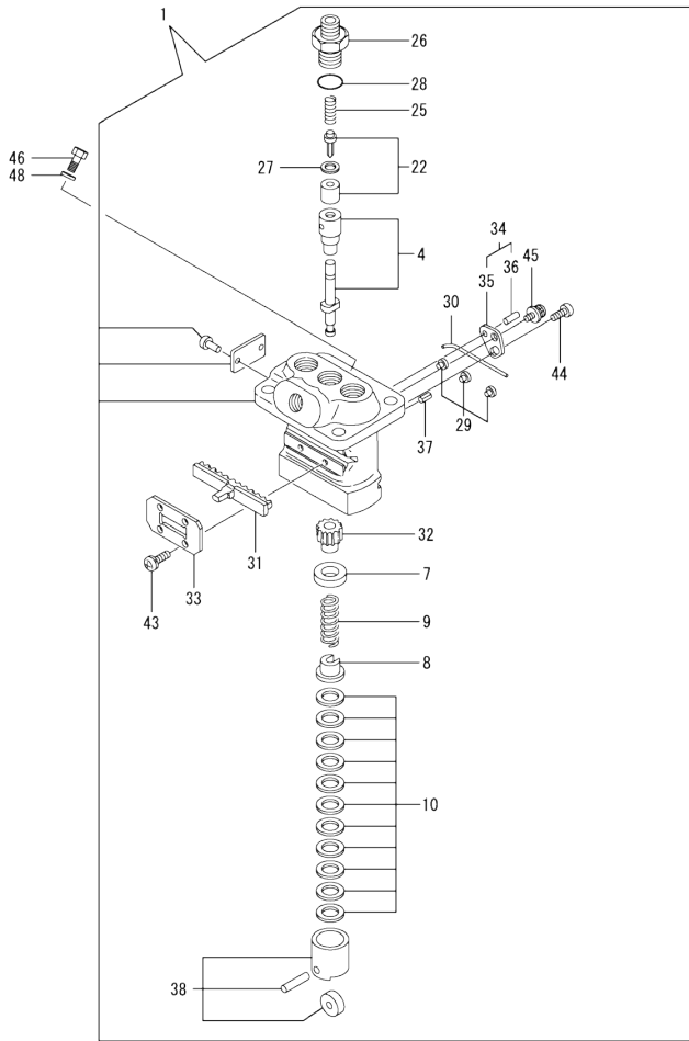
Fig.11. FUEL INJECTION PUMP
