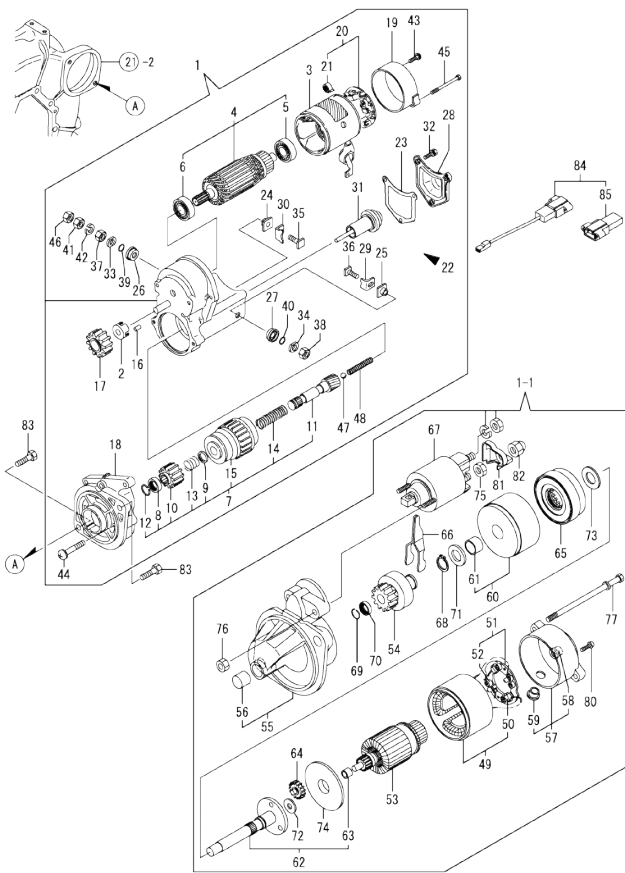
Fig.33. STARTING MOTOR
