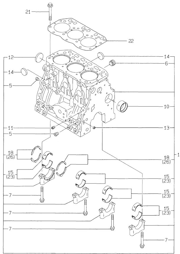
37.CYLINDER BLOCK
