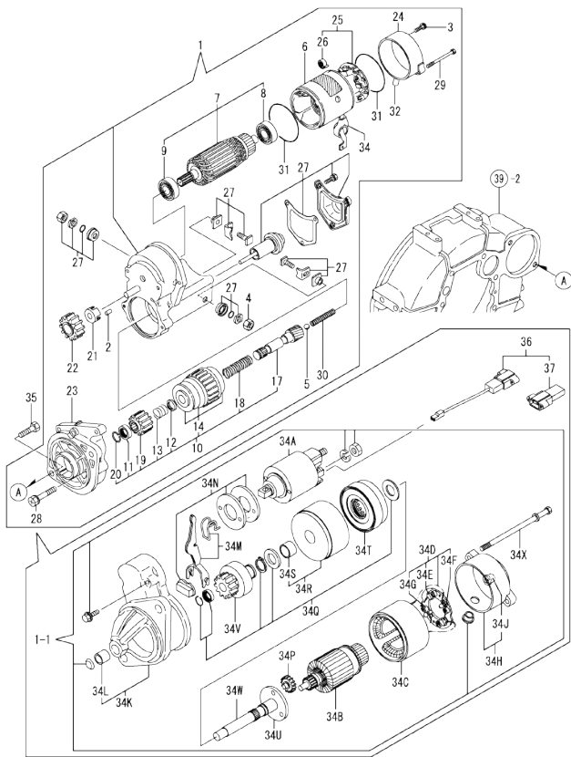
Fig.51. STARTING MOTOR
