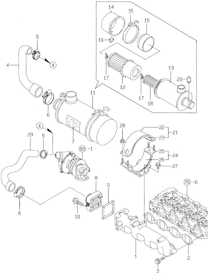
77.SUCTION MANIFOLD & AIR CLEANER
