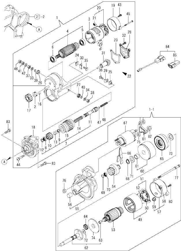
Fig.33. STARTING MOTOR
