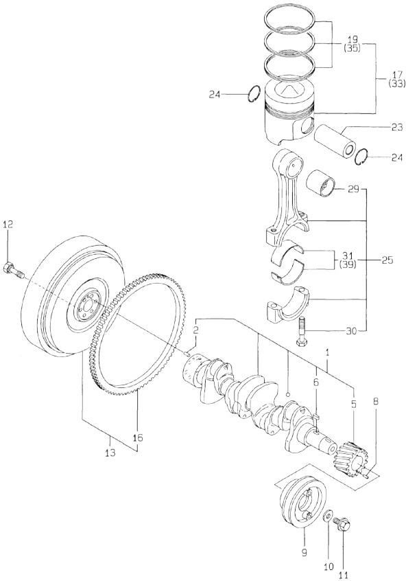
62.CRANKSHAFT & PISTON
