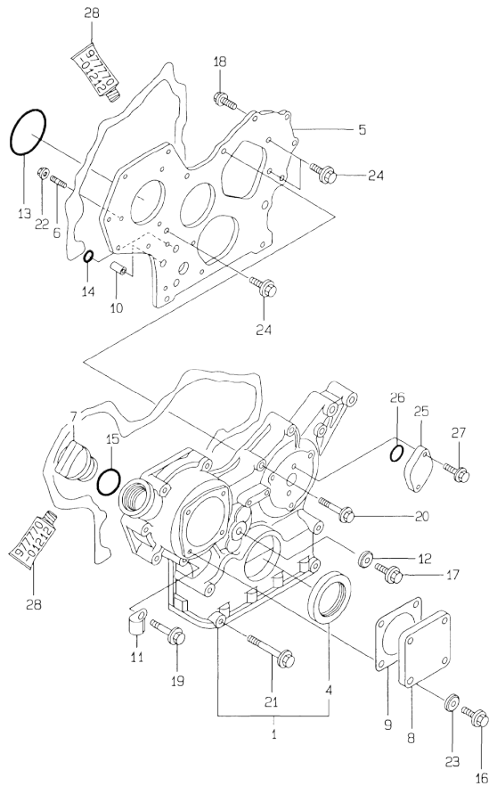
38. GEAR HOUSING
