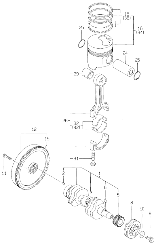
Fig.26. CRANKSHAFT & PISTON
