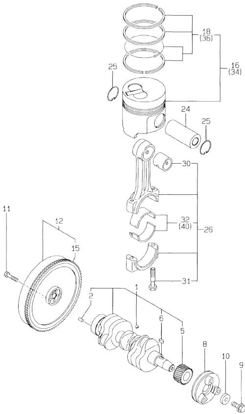
Fig.8. CRANKSHAFT & PISTON
