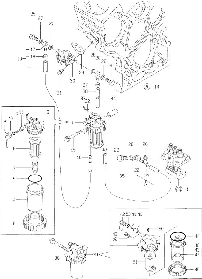
Fig.32. FUEL LINE
