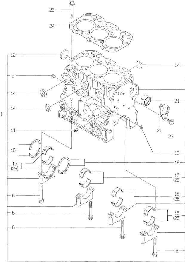
19. CYLINDER BLOCK
