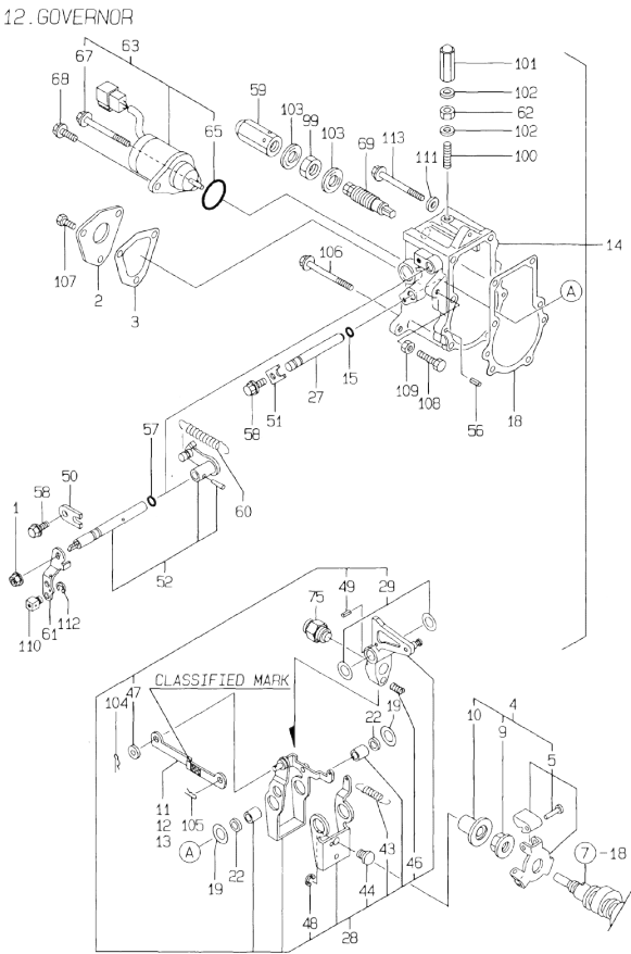
Fig.12. GOVERNOR
