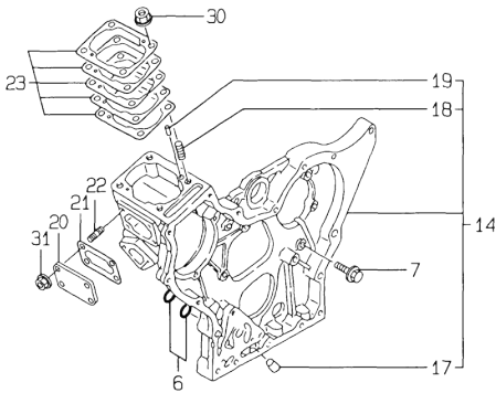
Fig.20. GEAR HOUSING
