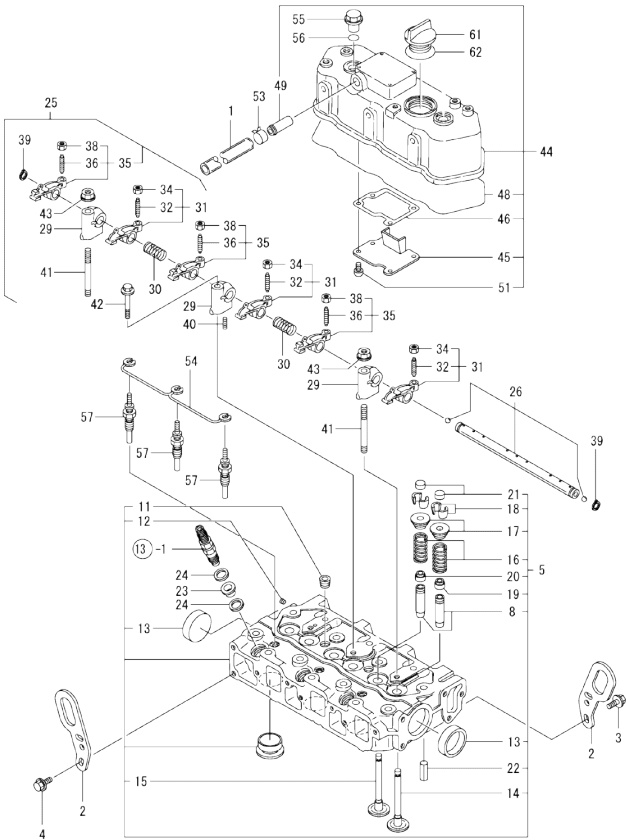
Fig.4. CYLINDER HEAD & BONET
