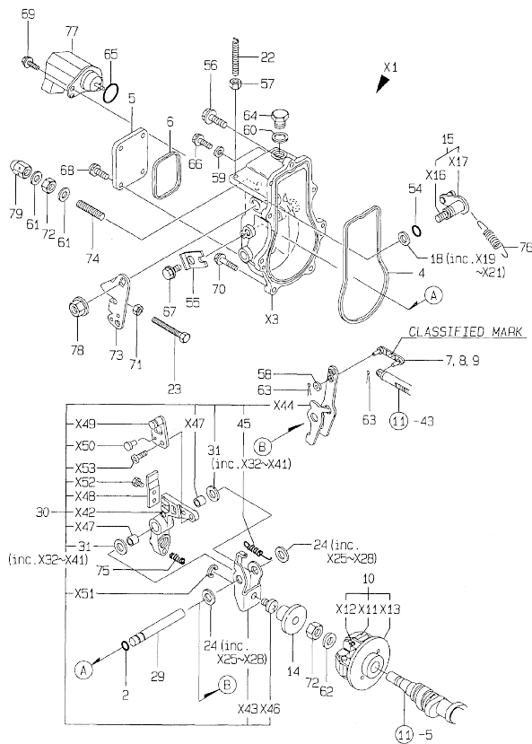
Fig.12. GOVERNOR
