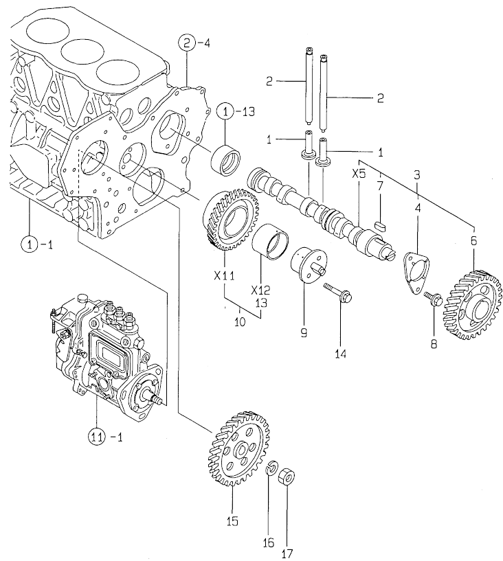
Fig.7. CAMSHAFT & DRIVING GEAR
