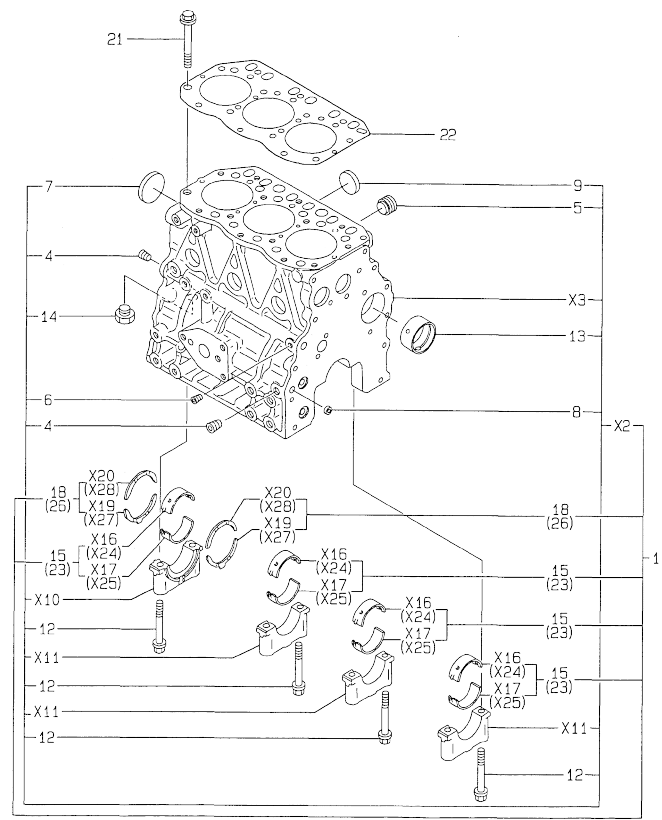
0CV10-M41200 3TNE78A-ADCL Fig.1. CYLINDER BLOCK
