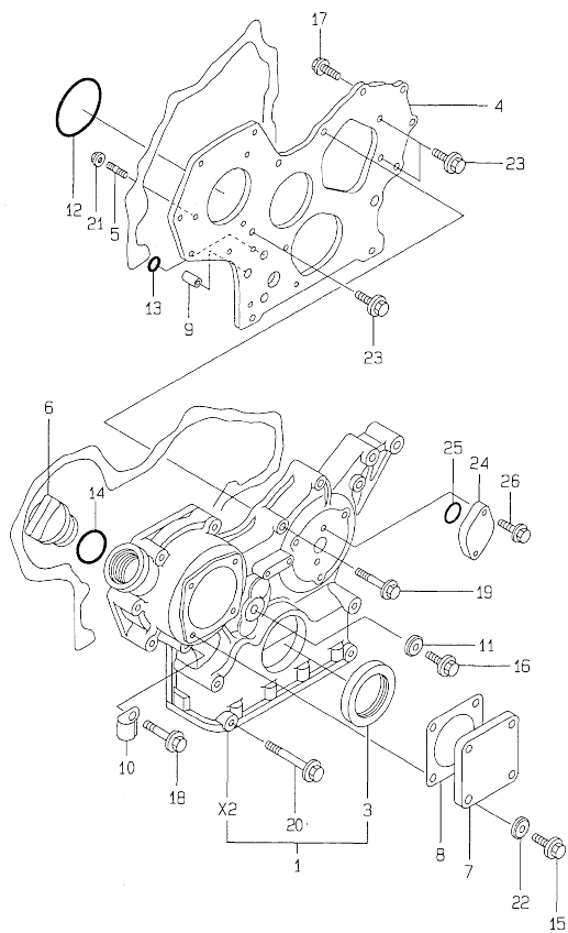
Fig.2. GEAR HOUSING
