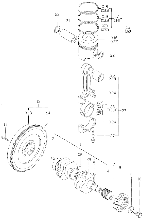
Fig.8. CRANKSHAFT & PISTON
