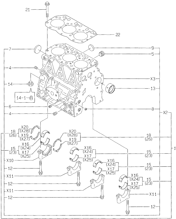
Fig.1. CYLINDER BLOCK
