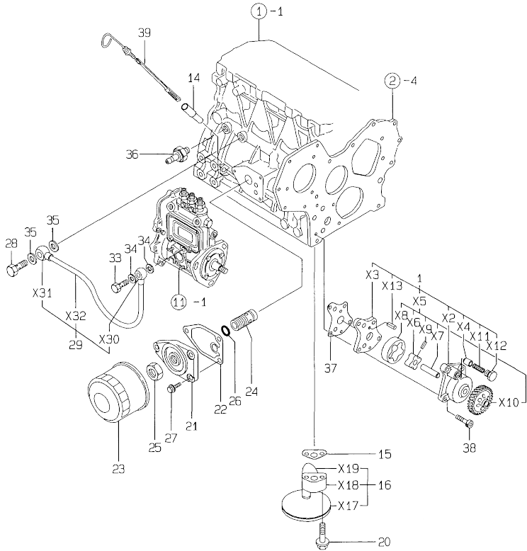
Fig.9. LUB.OIL SYSTEM
