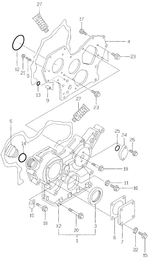
2. GEAR HOUSING
