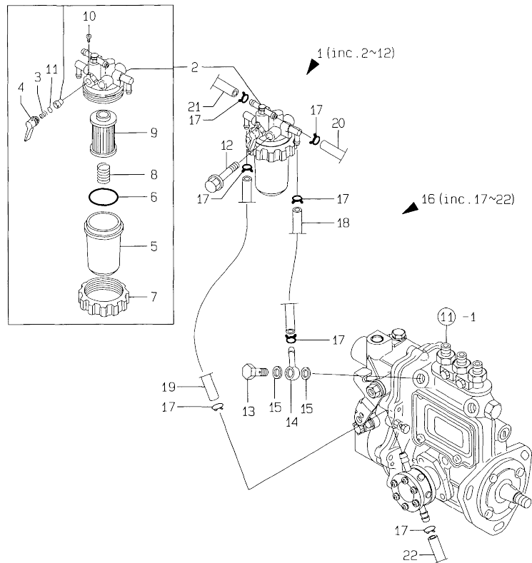
Fig.14. FUEL LINE
