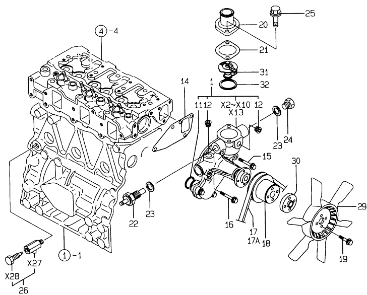
Fig.9. COOLING WATER SYSTEM
