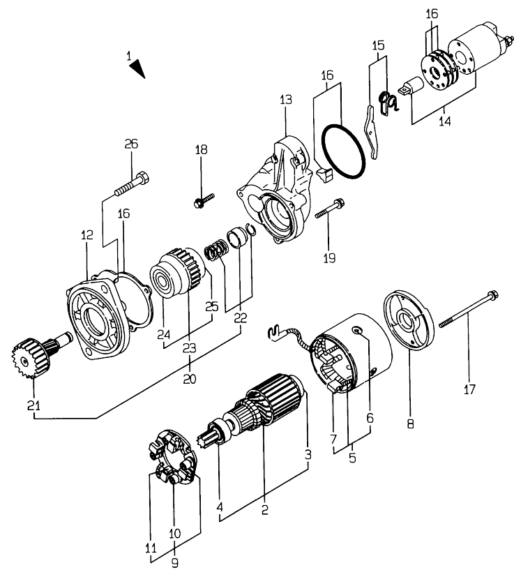
Fig.14. STARTING MOTOR
