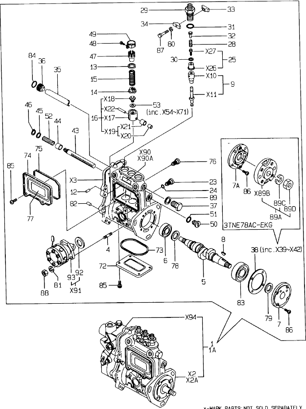
10.FUEL INJECTION PUMP
