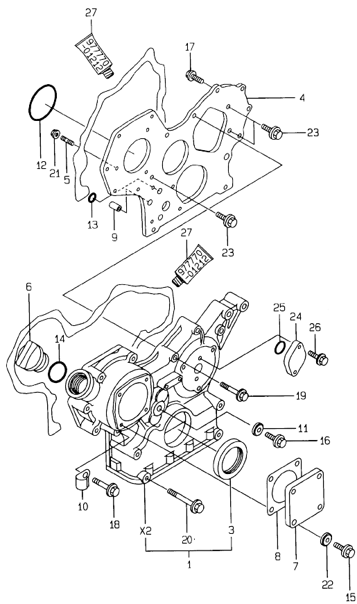
Fig.2. GEAR HOUSING
