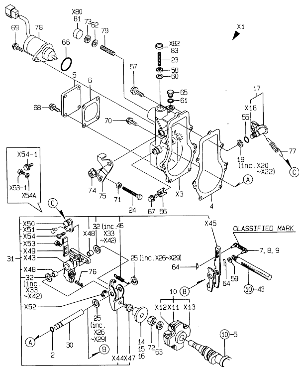
Fig.11. GOVERNOR
