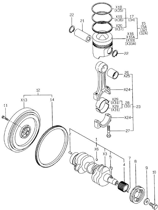
Fig.7. CRANKSHAFT & PISTON
