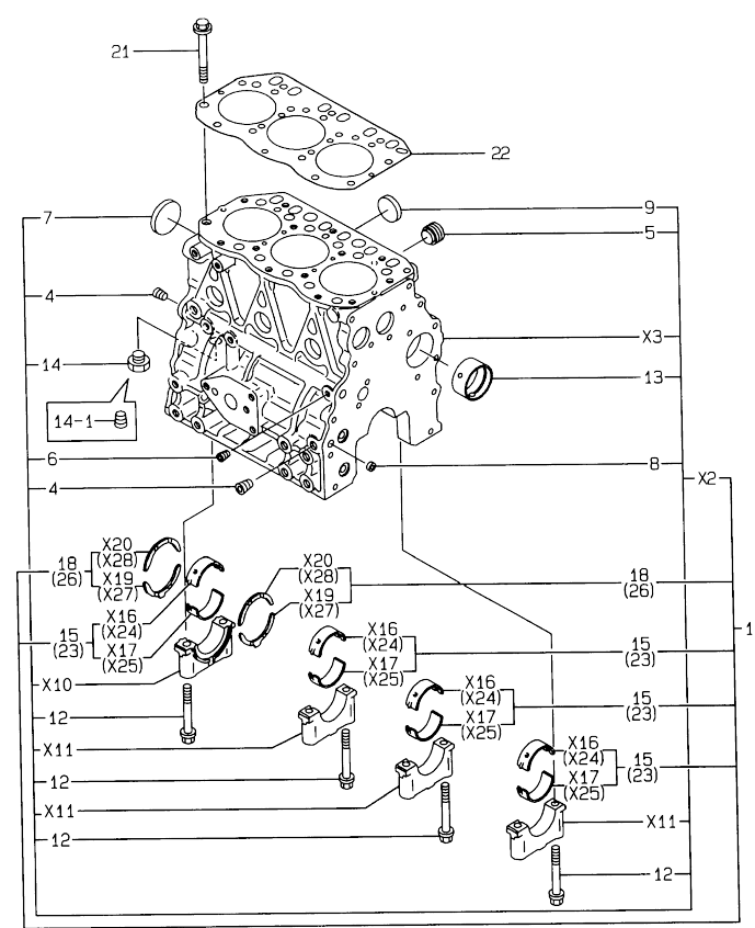
Fig.1. CYLINDER BLOCK
