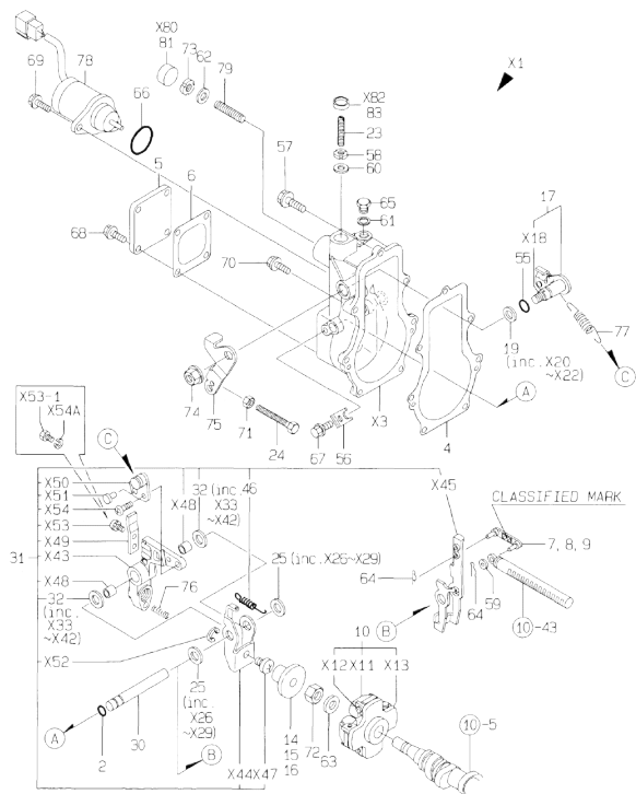
11. GOVERNOR
