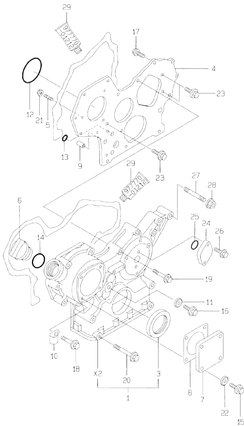
2. GEAR HOUSING
