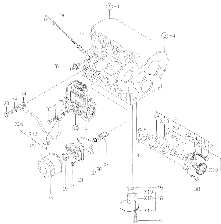
Fig.8. LUB.OIL SYSTEM
