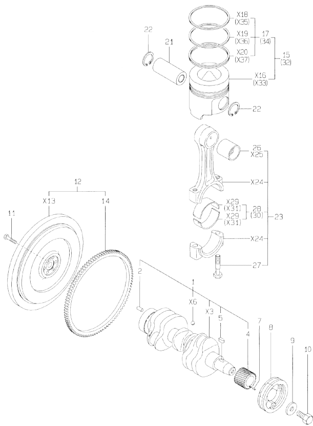
Fig.7. CRANKSHAFT & PISTON
