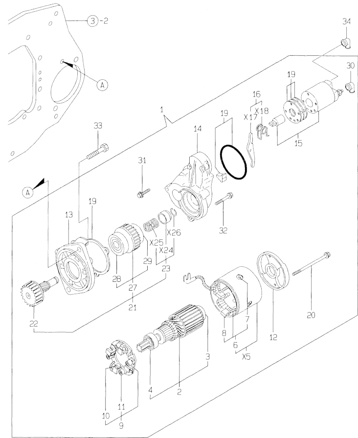
Fig.14. STARTING MOTOR
