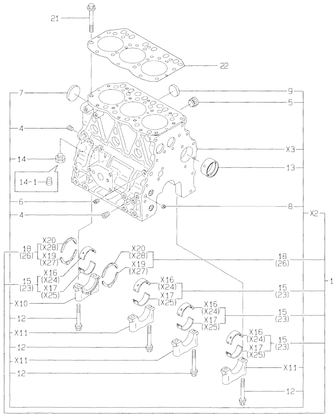
Fig.1. CYLINDER BLOCK
