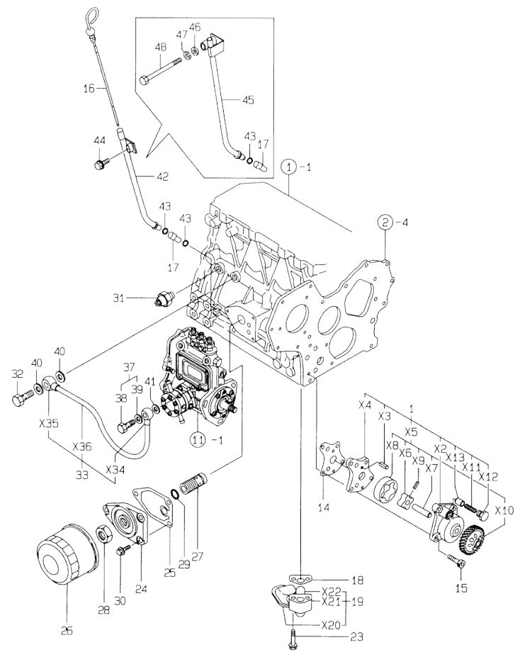
Fig.9. LUB.OIL SYSTEM
