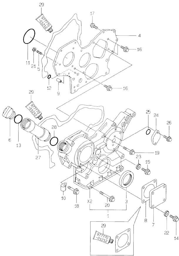
Fig.2. GEAR HOUSING
