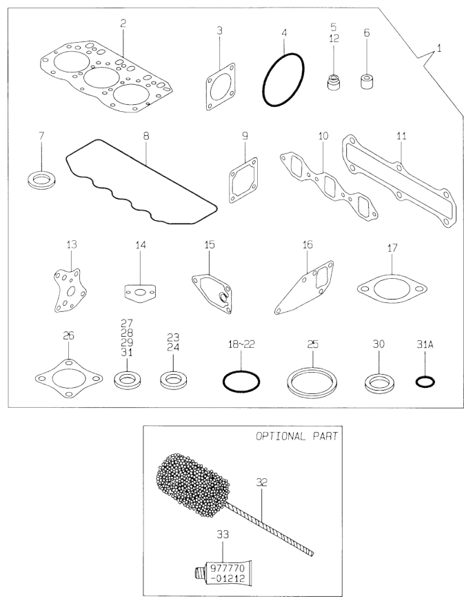
Fig.17. GASKET SET
