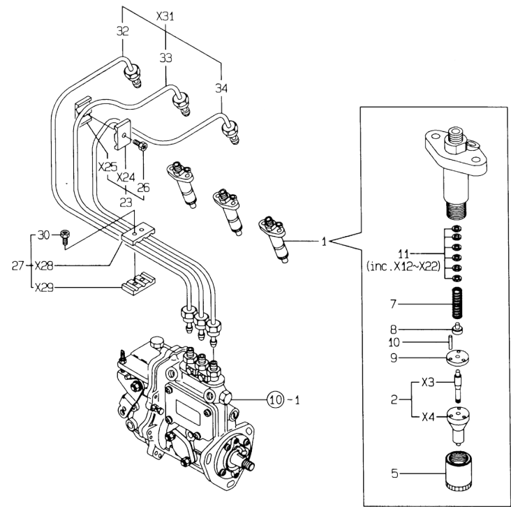
Fig.12. FUEL INJECTION VALVE
