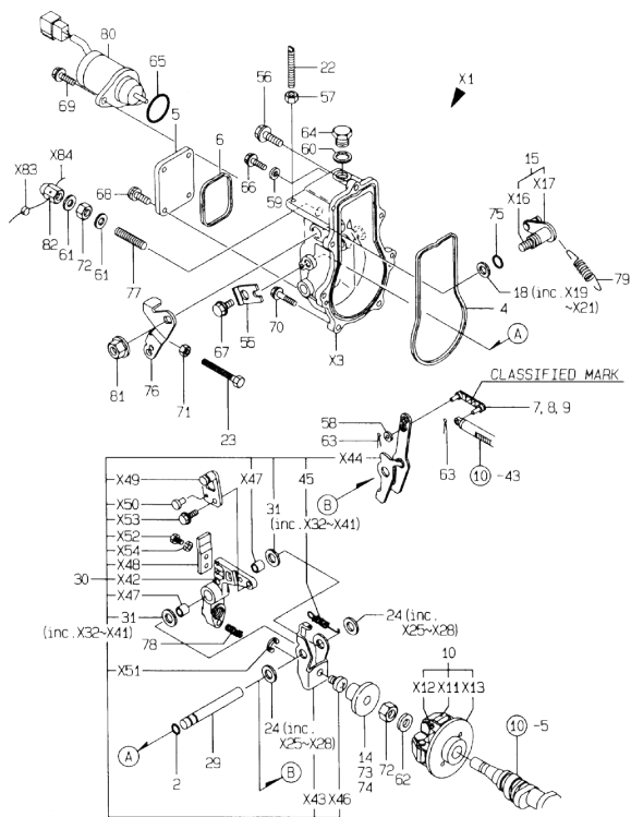
Fig.11. GOVERNOR
