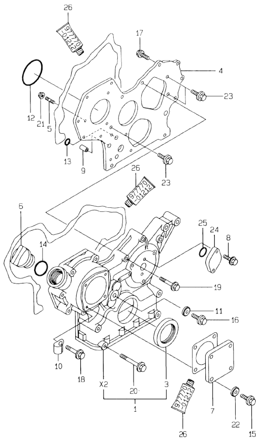
2. GEAR HOUSING
