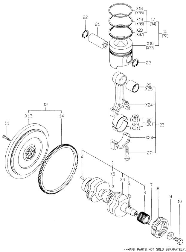
Fig.7. CRANKSHAFT & PISTON
