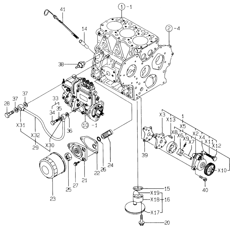
Fig.8. LUB.OIL SYSTEM
