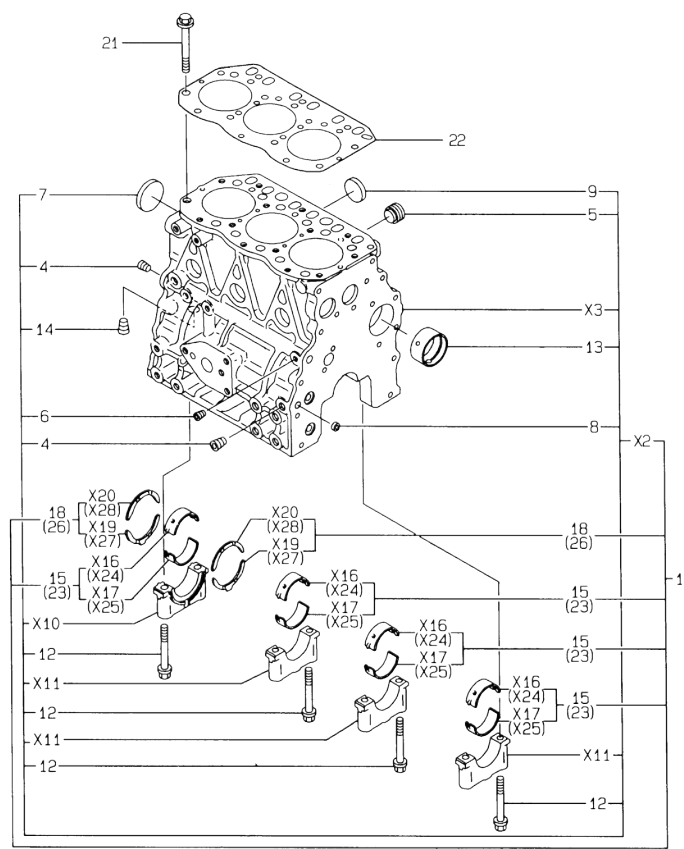
Fig.1. CYLINDER BLOCK
