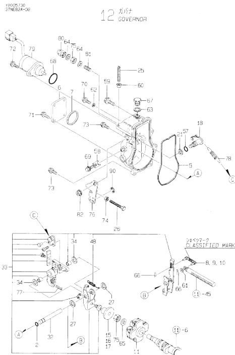
Fig.12. GOVERNOR
