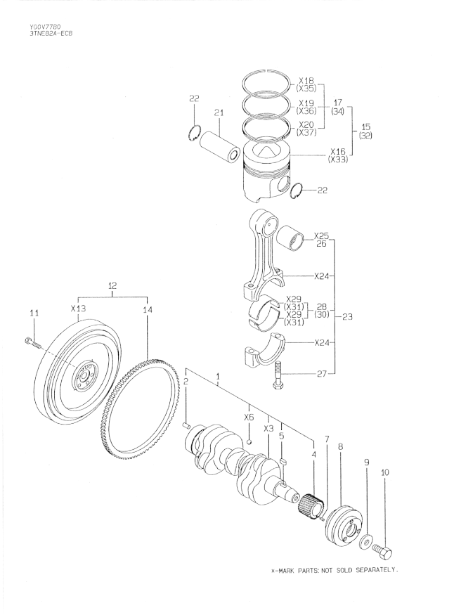
Fig.8. CRANKSHAFT & PISTON
