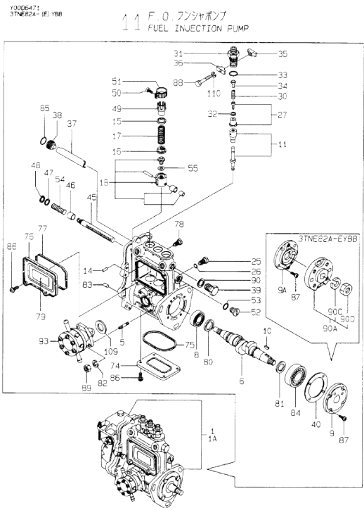
OCD10-M64701 3TNE82A-(E)YBB Fig.11. FUEL INJECTION PUMP
