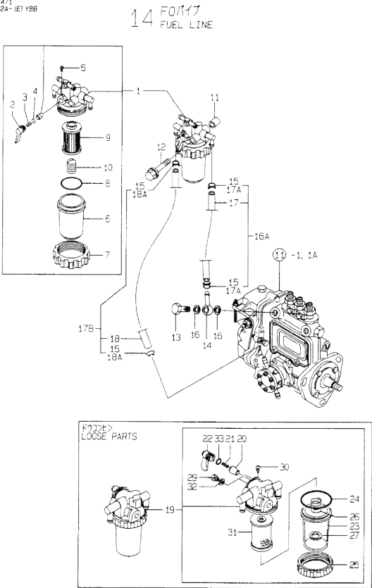
OCD10-M64701 3TNE82A-(E)YBB Fig.14. FUEL LINE
