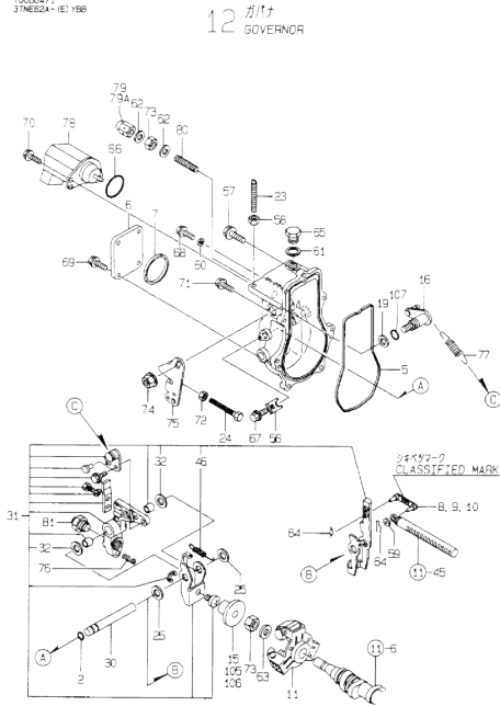
Fig.12. GOVERNOR
