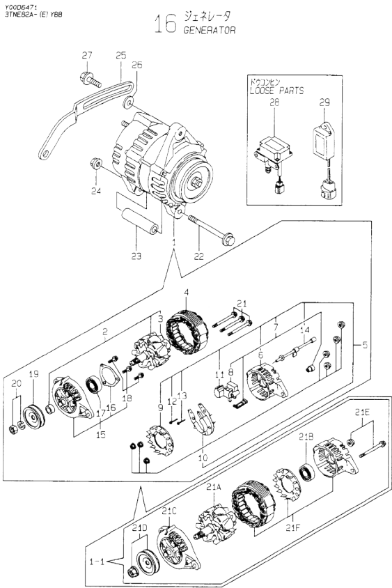
OCD10-M64701 3TNE82A-(E)YBB Fig.16. GENERATOR
