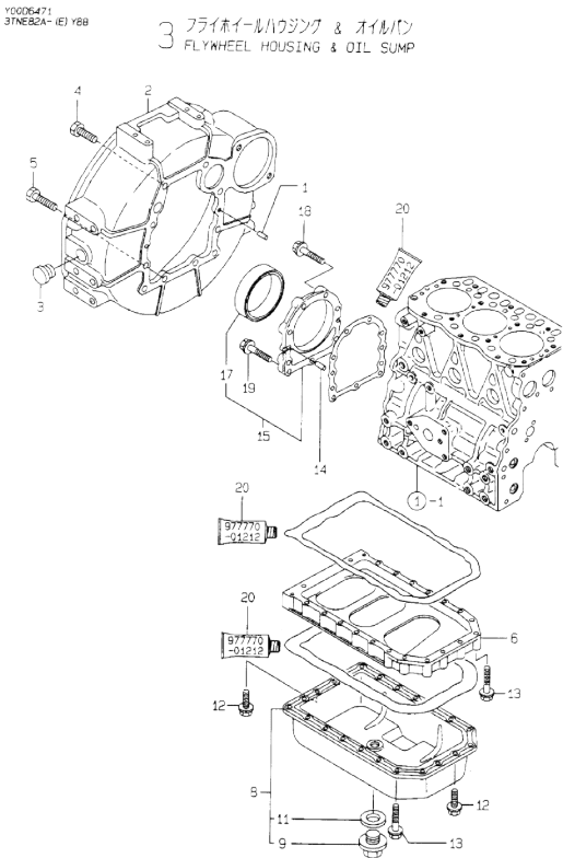
Fig.3. FLYWHEEL HOUSING & OIL SUMP
