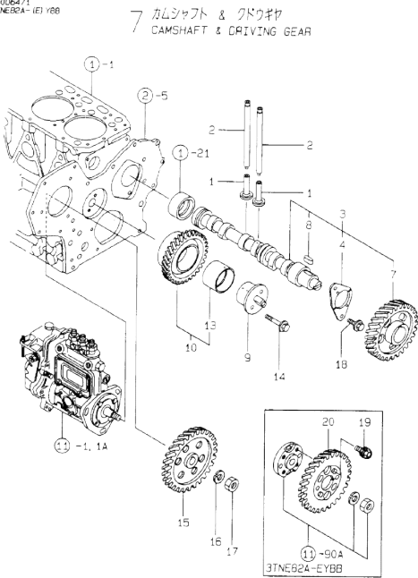
Fig.7. CAMSHAFT & DRIVING GEAR
