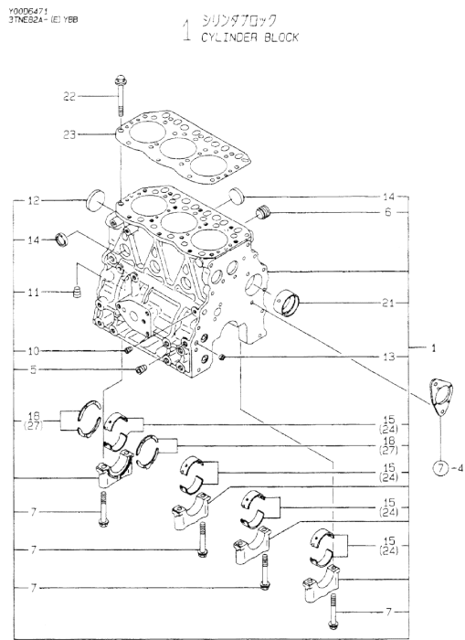
OCD10-M64701 3TNE82A-(E)YBB Fig.1. CYLINDER BLOCK
