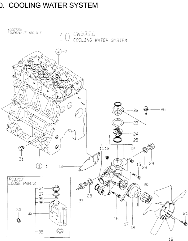
Fig.10. COOLING WATER SYSTEM
