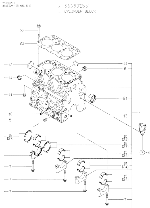
Fig.1. CYLINDER BLOCK
