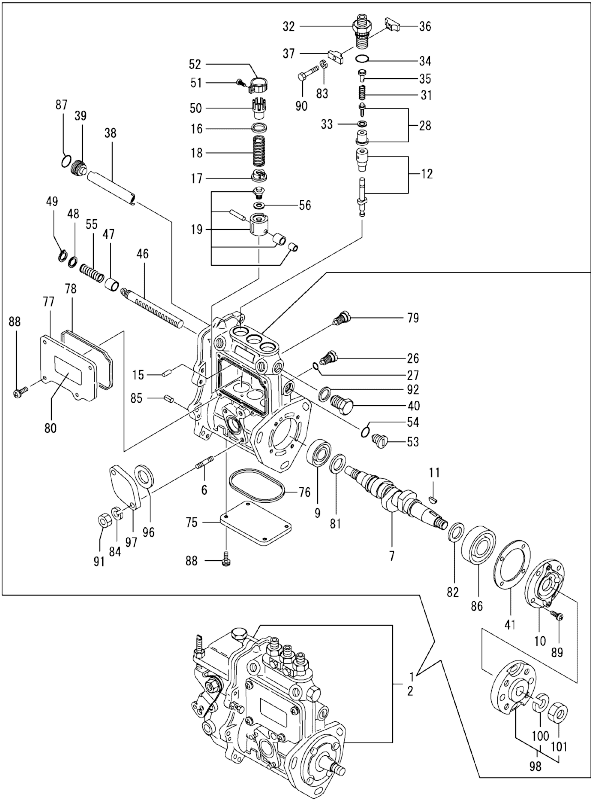
OCD10-M72701 ENGINE SECTION Fig.11. FUEL INJECTION PUMP
