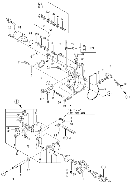
Fig.12. GOVERNOR
