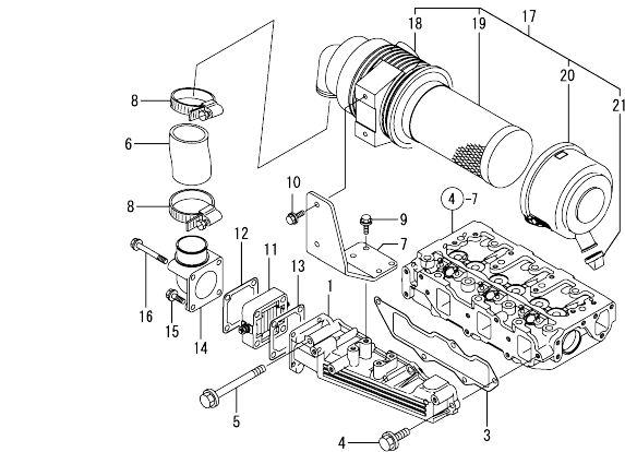
Fig.5. SUCTION MANIFOLD & AIR CLEANER
