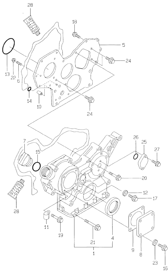
56. GEAR HOUSING
