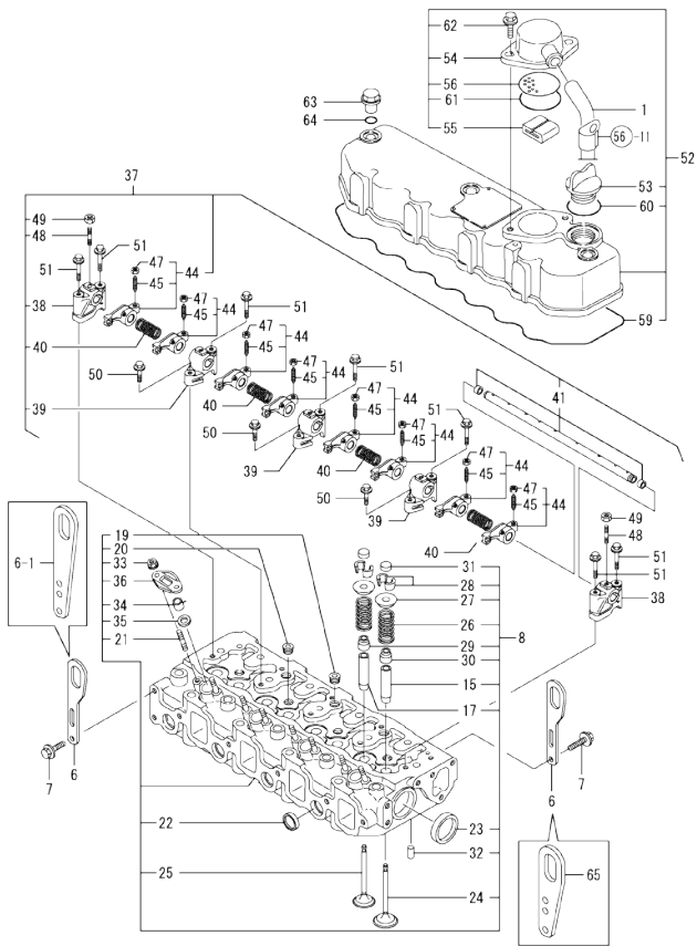
Fig.58. CYLINDER HEAD & BONNET
