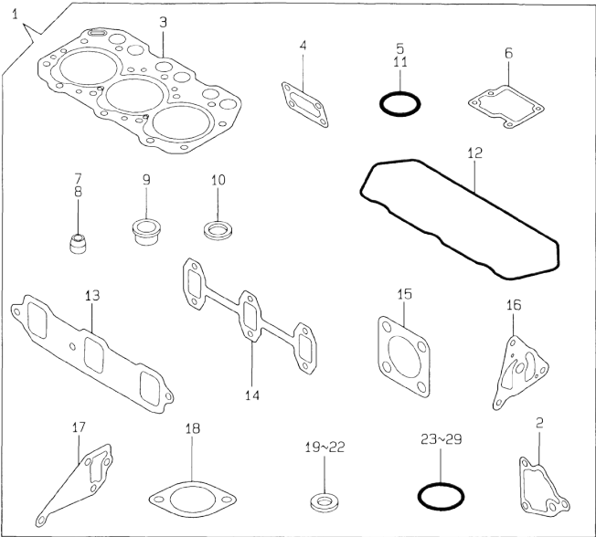
Fig.36. GASKET SET & TOOLS
