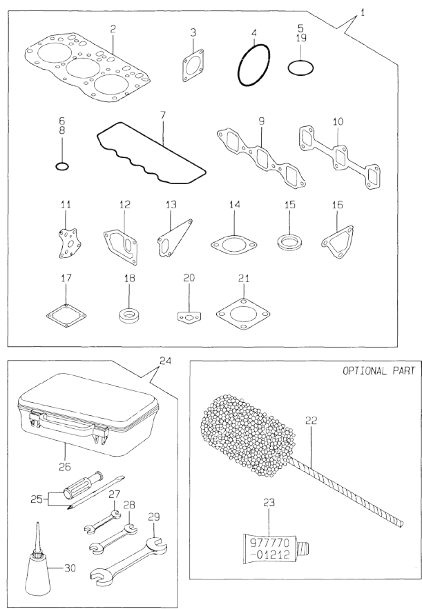
Fig.54. GASKET SET & TOOLS
