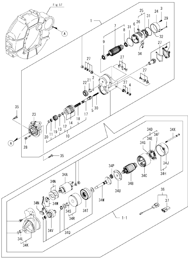
Fig.69. STARTING MOTOR
