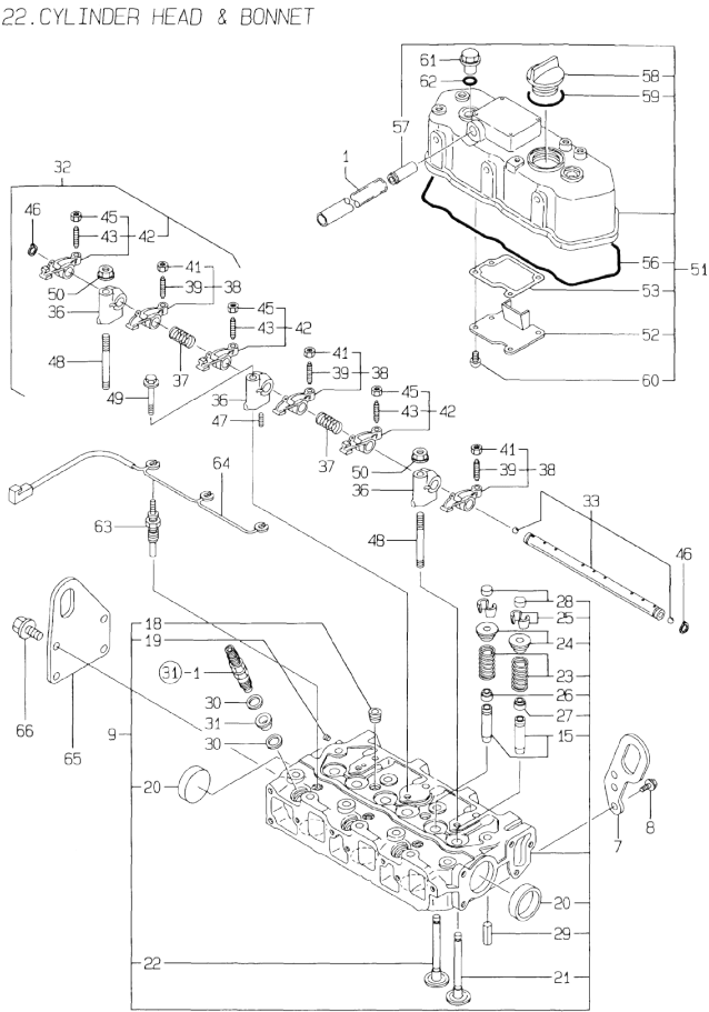
Fig.22. CYLINDER HEAD & BONNET
