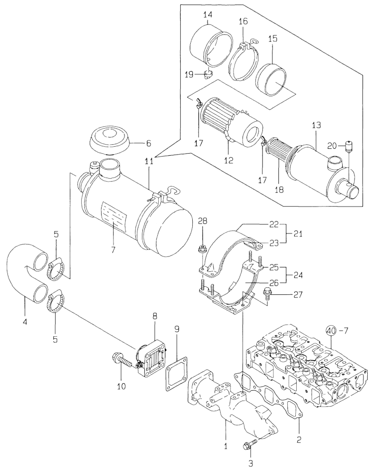
Fig.41. SUCTION MANIFOLD & AIR CLEANER
