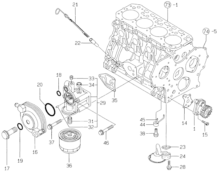
OCB10-M60200 4TNE84T-GB2S Fig.82. LUB. OIL SYSTEM
