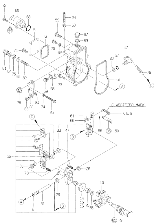
86. GOVERNOR
