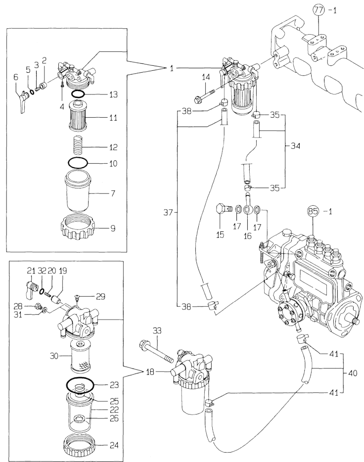
Fig.88. FUEL LINE
