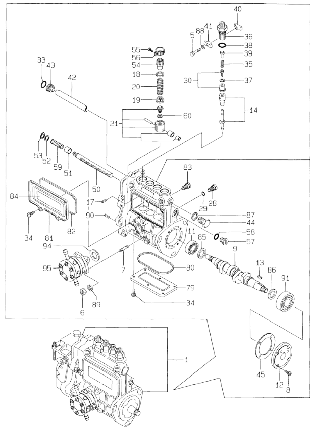
85.FUEL INJECTION PUMP
