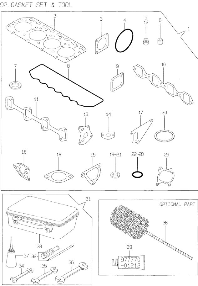
Fig.92. GASKET SET & TOOLS
