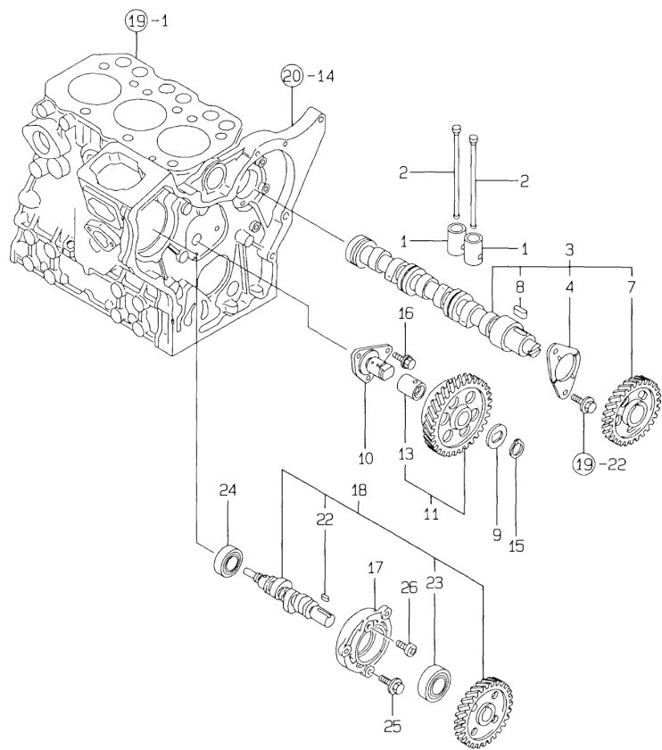
Fig.25. CAMSHAFT & DRIVING GEAR
