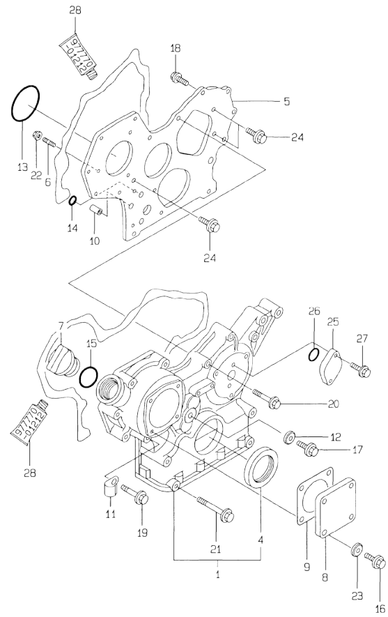
38. GEAR HOUSING
