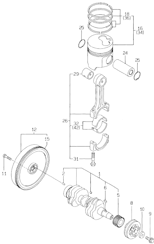
Fig.26. CRANKSHAFT & PISTON
