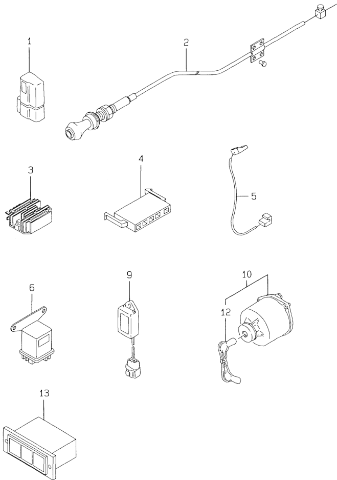
Fig.91. ELECTRICAL PARTS
