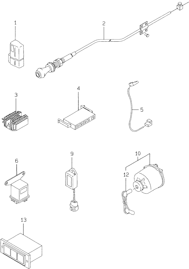
Fig.71. ELECTRICAL PARTS
