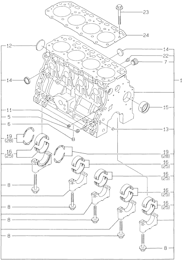
73.CYLINDER BLOCK
