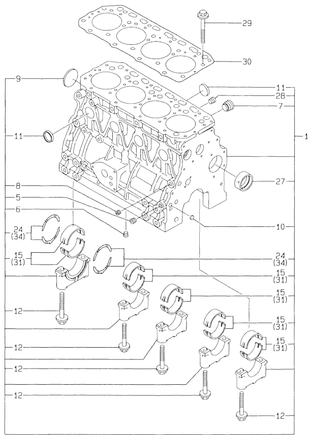
Fig.55. CYLINDER BLOCK
