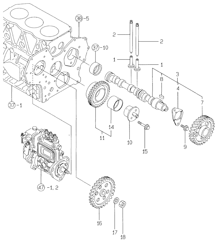
Fig.43. CAMSHAFT & DRIVING GEAR
