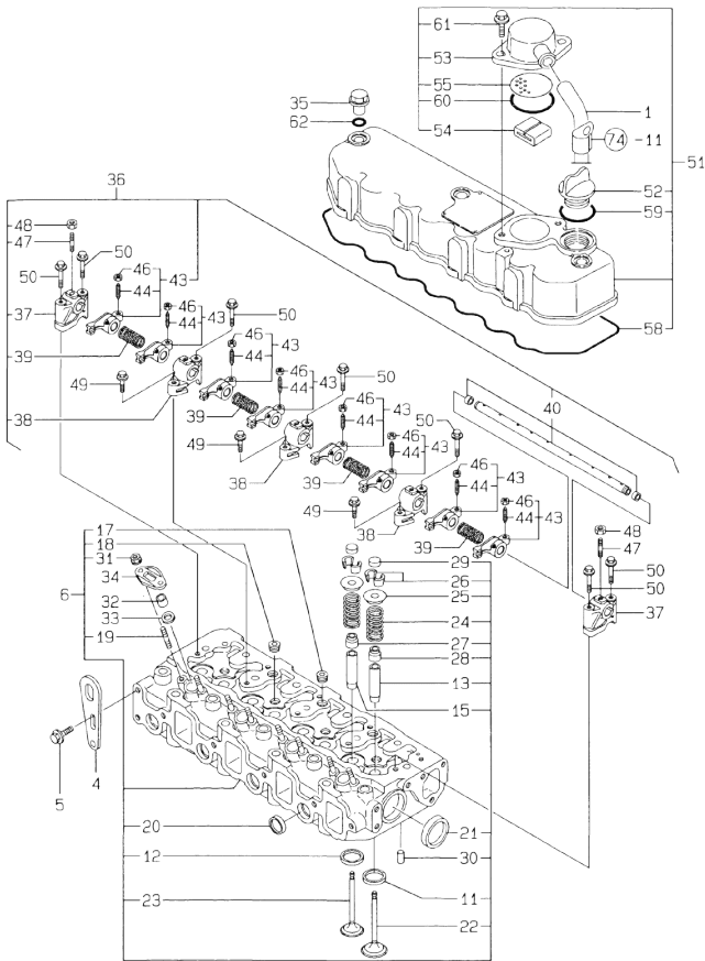
76.CYLINDER HEAD & BONNET
