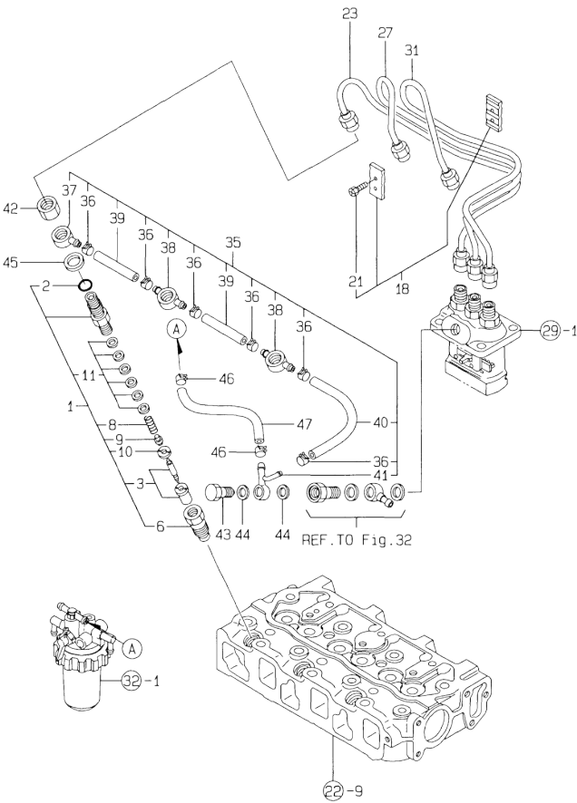
Fig.31. FUEL INJECTION VALVE
