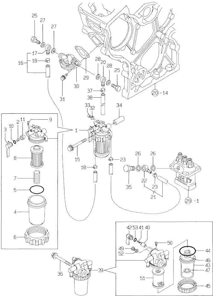
Fig.32. FUEL LINE
