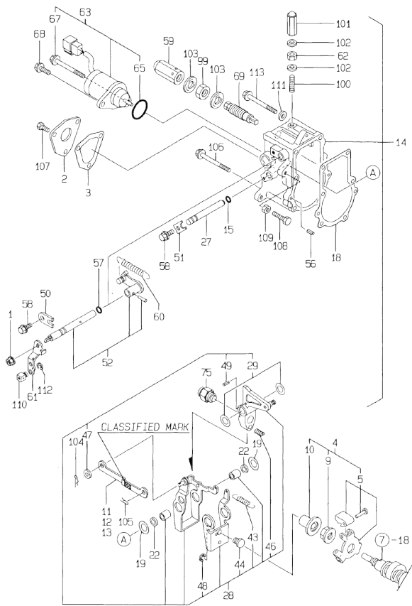
Fig.12. GOVERNOR
