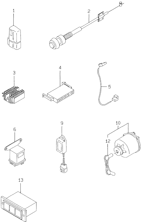
Fig.17. ELECTRICAL PARTS
