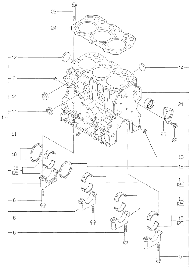
19. CYLINDER BLOCK
