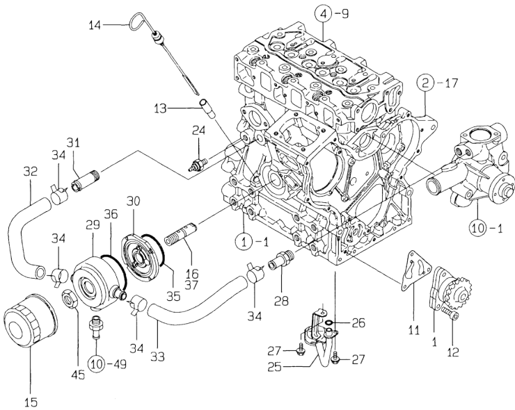
Fig.9. LUB. OIL SYSTEM
