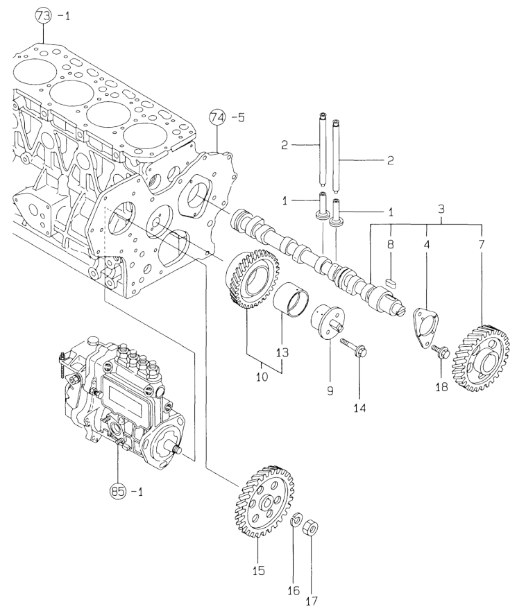
Fig.79. CAMSHAFT & DRIVING GEAR
