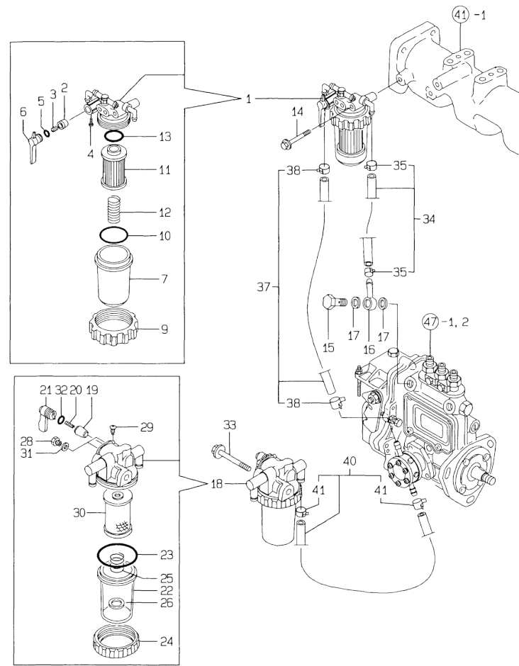
Fig.50. FUEL LINE
