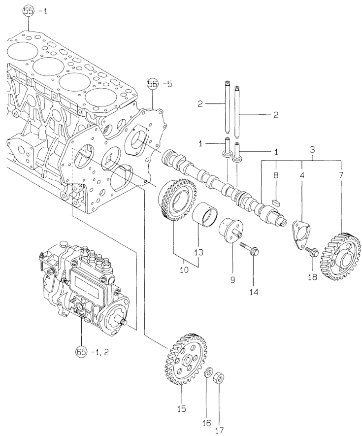
Fig.61. CAMSHAFT & DRIVING GEAR
