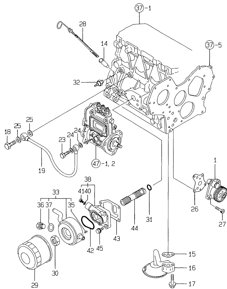
Fig.45. LUB. OIL SYSTEM
