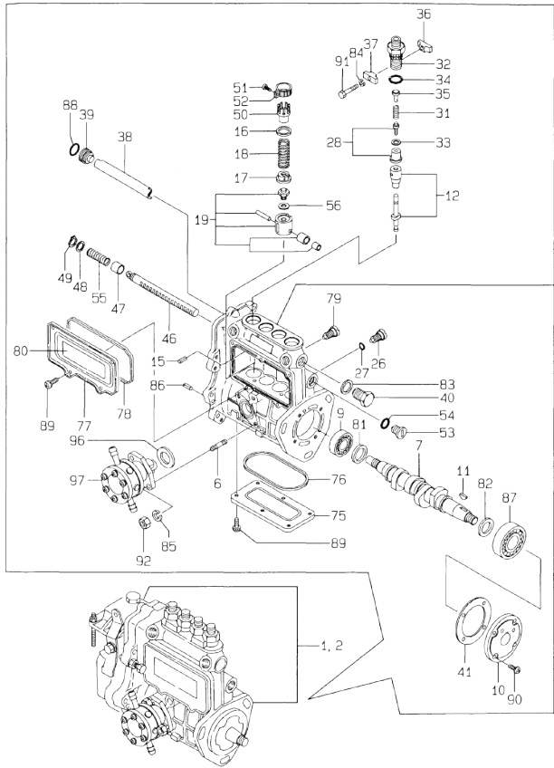
65.FUEL INJECTION PUMP
