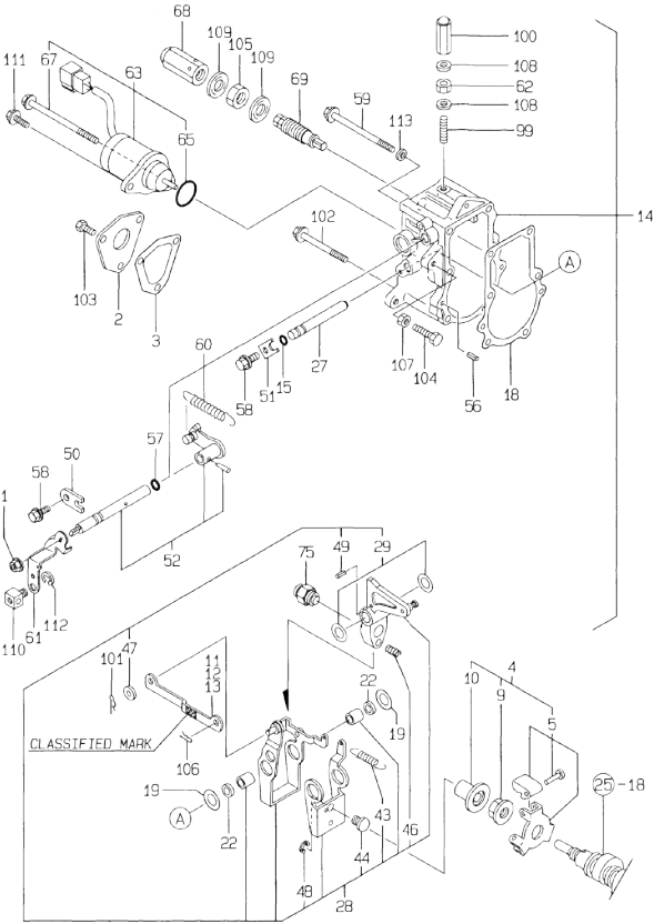
Fig.30. GOVERNOR
