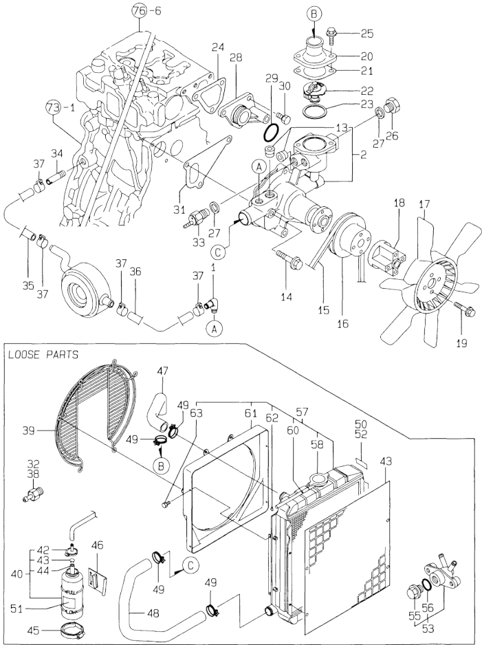
Fig.84. COOLING WATER SYSTEM
