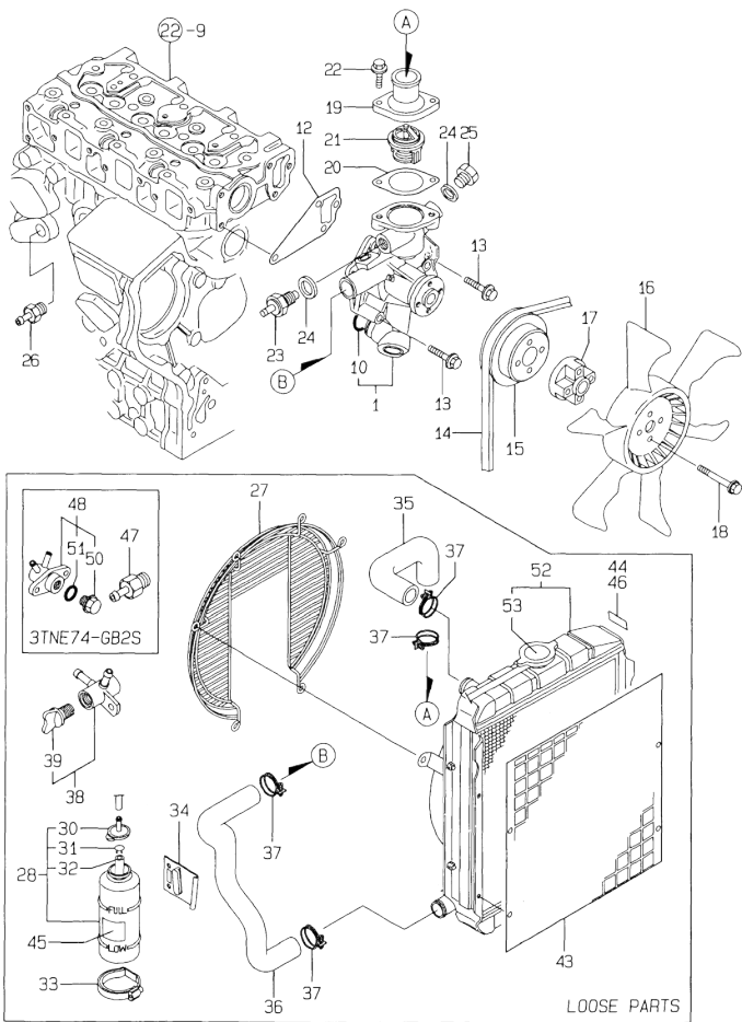
Fig.28. COOLING WATER SYSTEM
