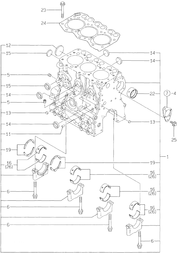
Fig.1. CYLINDER BLOCK
