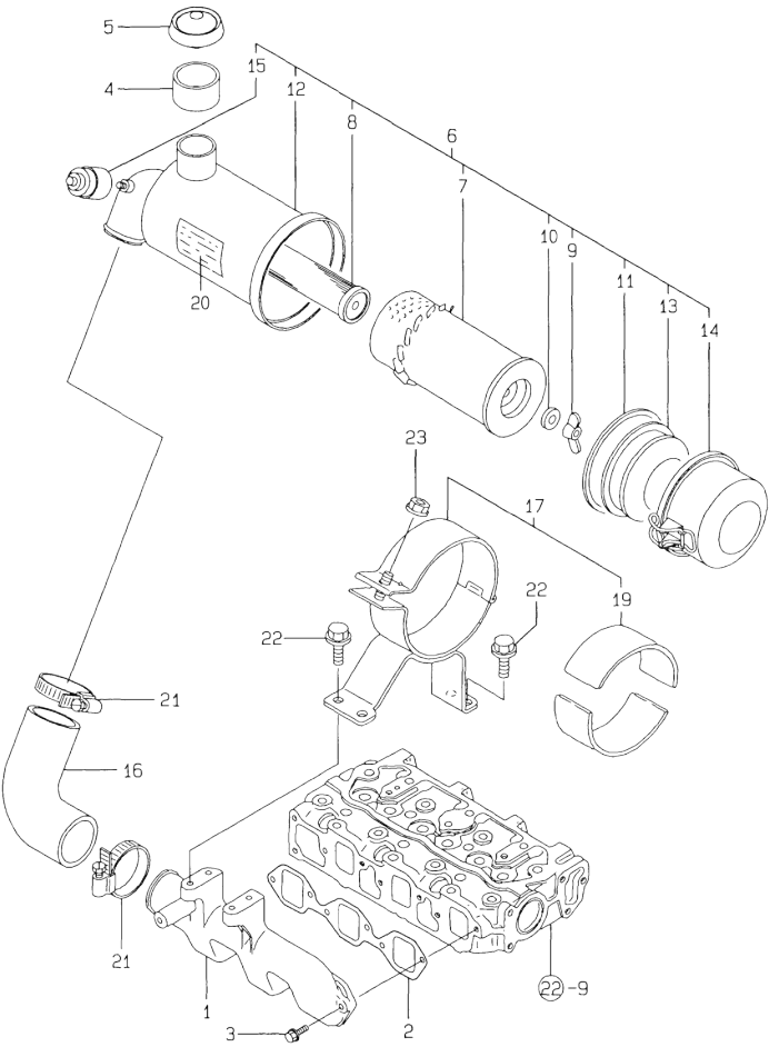
23.SUCTION MANIFOLD & AIR CLEANER
