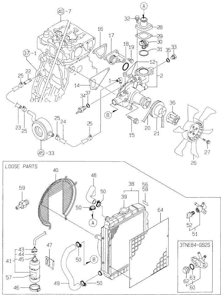
Fig.46. COOLING WATER SYSTEM
