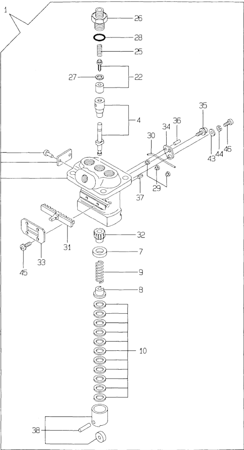
29.FUEL INJECTION PUMP
