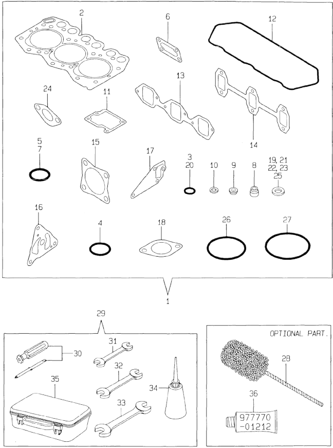
Fig.18. GASKET SET & TOOLS
