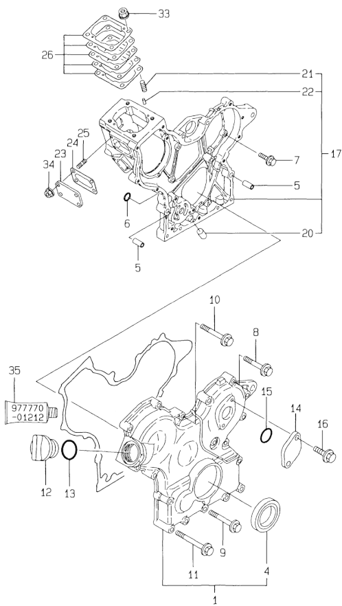
Fig.2. GEAR HOUSING
