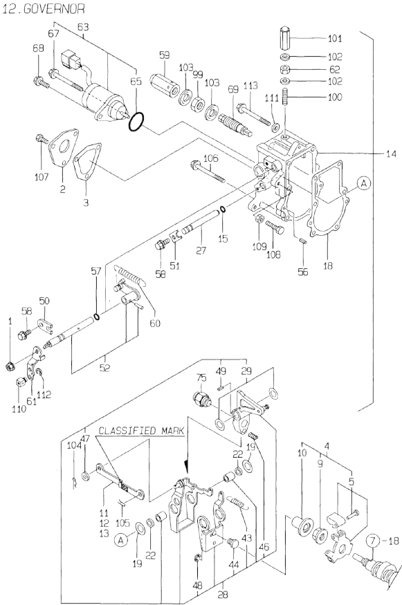
Fig.12. GOVERNOR
