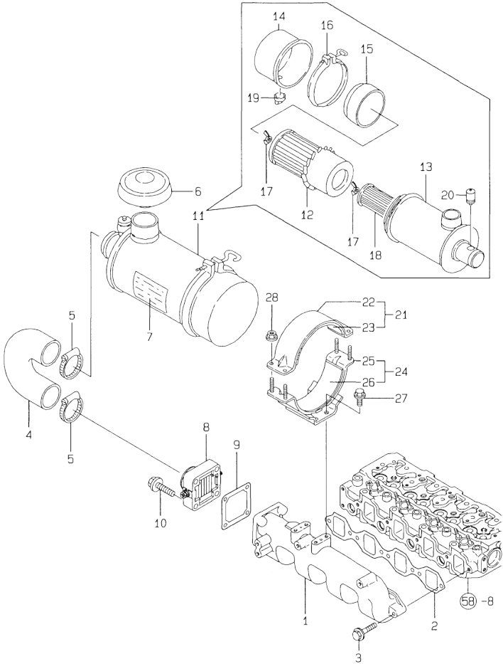
Fig.59. SUCTION MANIFOLD & AIR CLEANER
