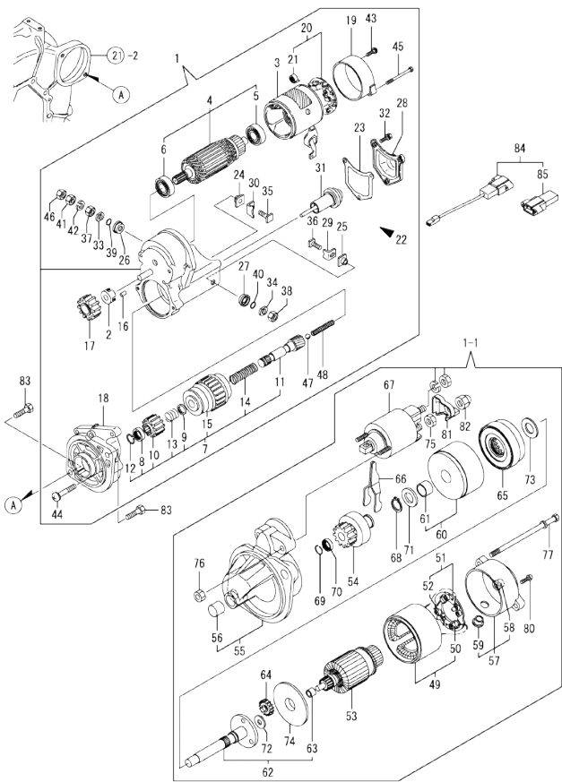
Fig.33. STARTING MOTOR
