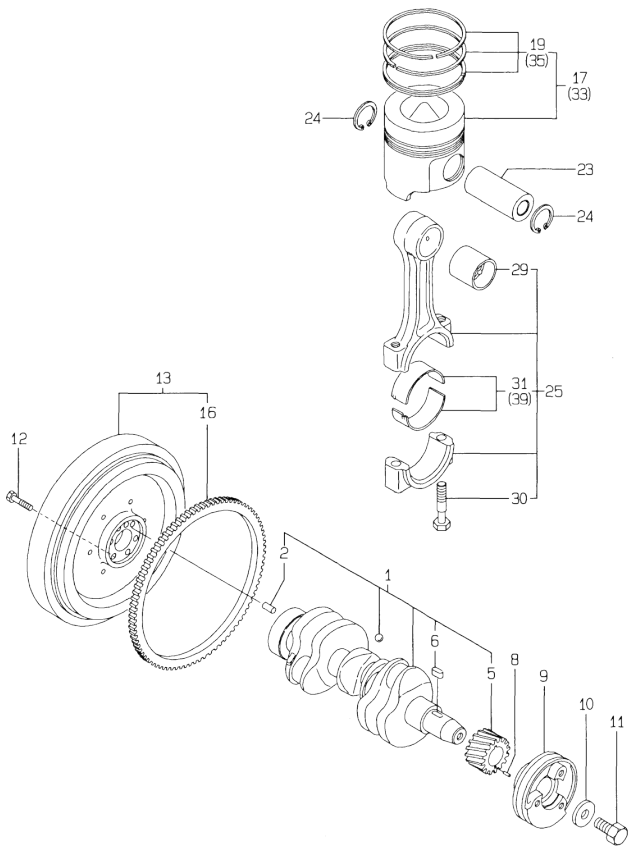
Fig.44. CRANKSHAFT & PISTON
