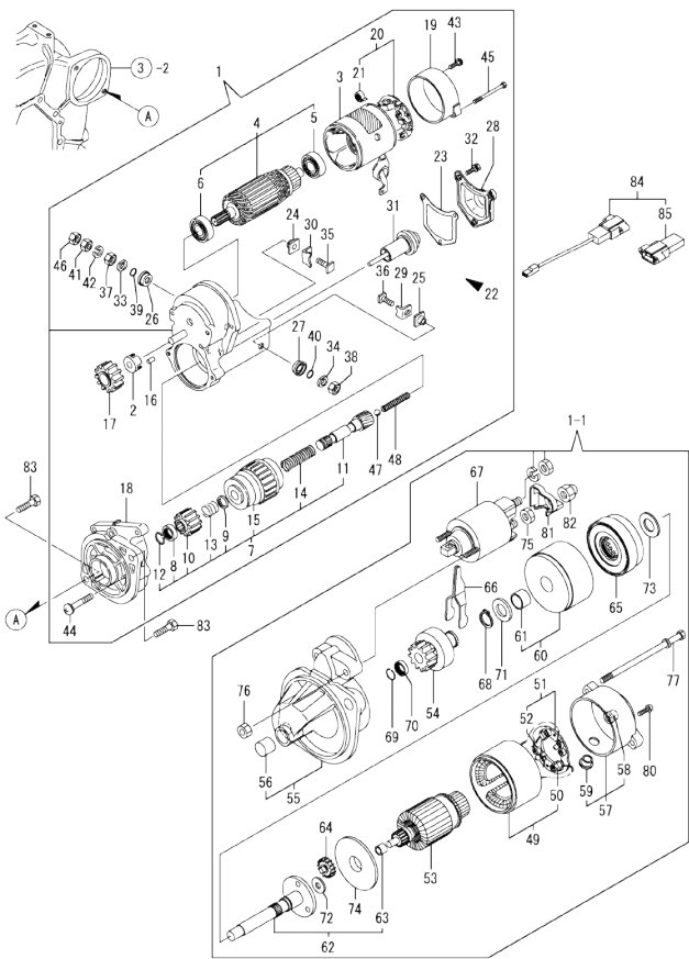
Fig.15. STARTING MOTOR
