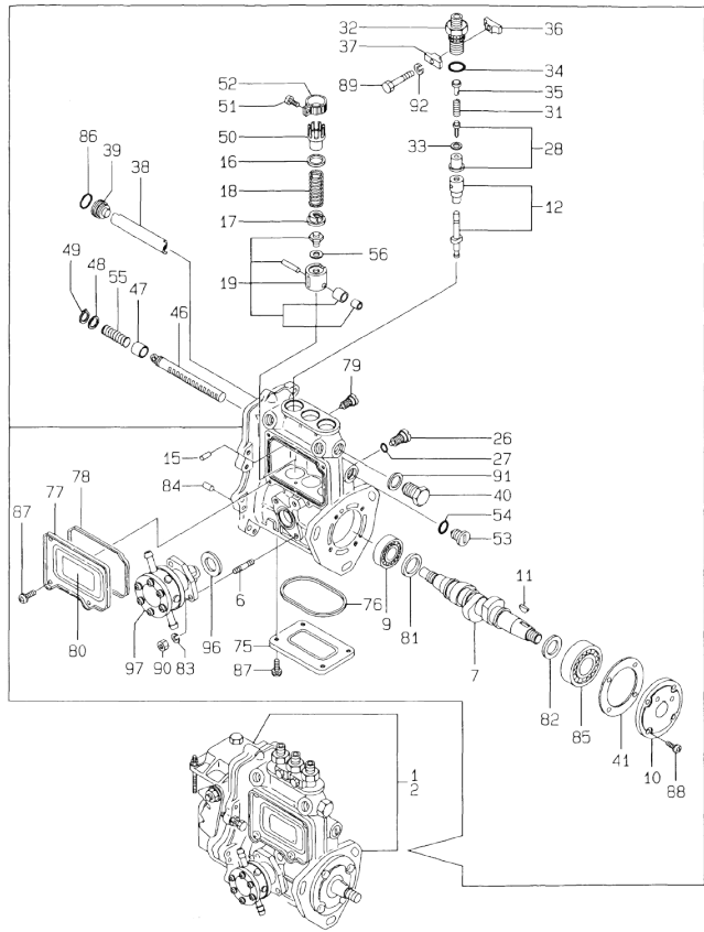
47.FUEL INJECTION PUMP
