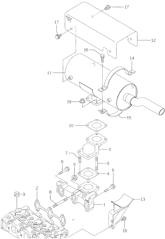
Fig.24. EXHAUST MANIFOLD & SILENCER
