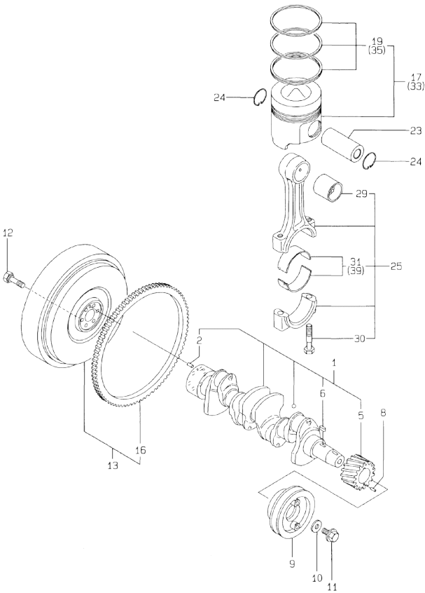
Fig.81. CRANKSHAFT & PISTON
