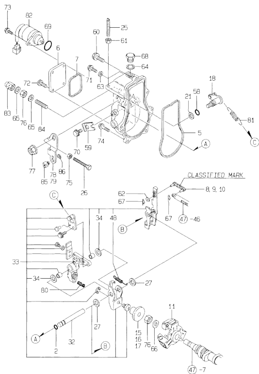
48. GOVERNOR
