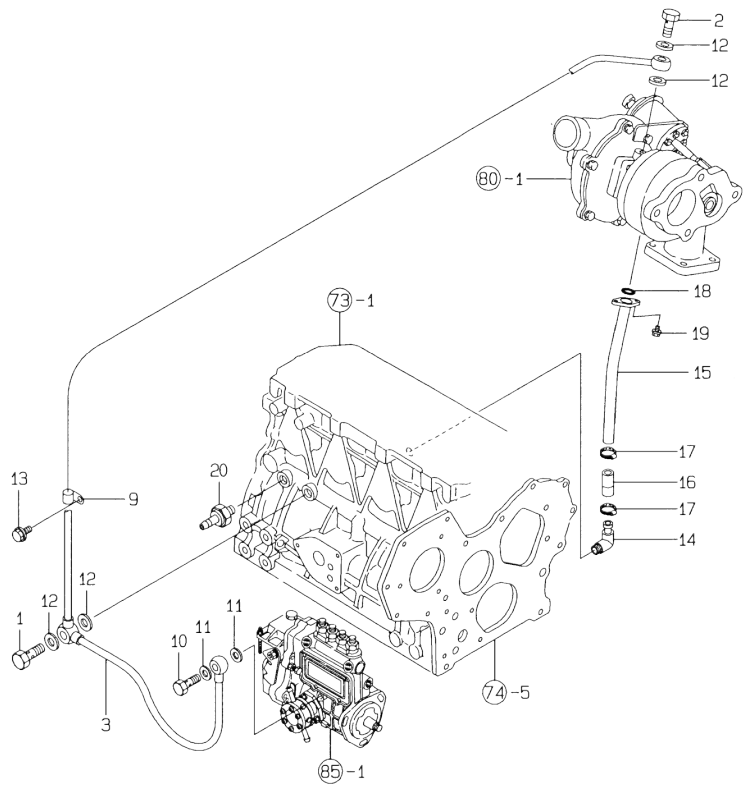
Fig.83. LUB. OIL LINE
