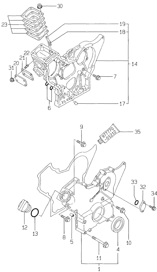
20. GEAR HOUSING
