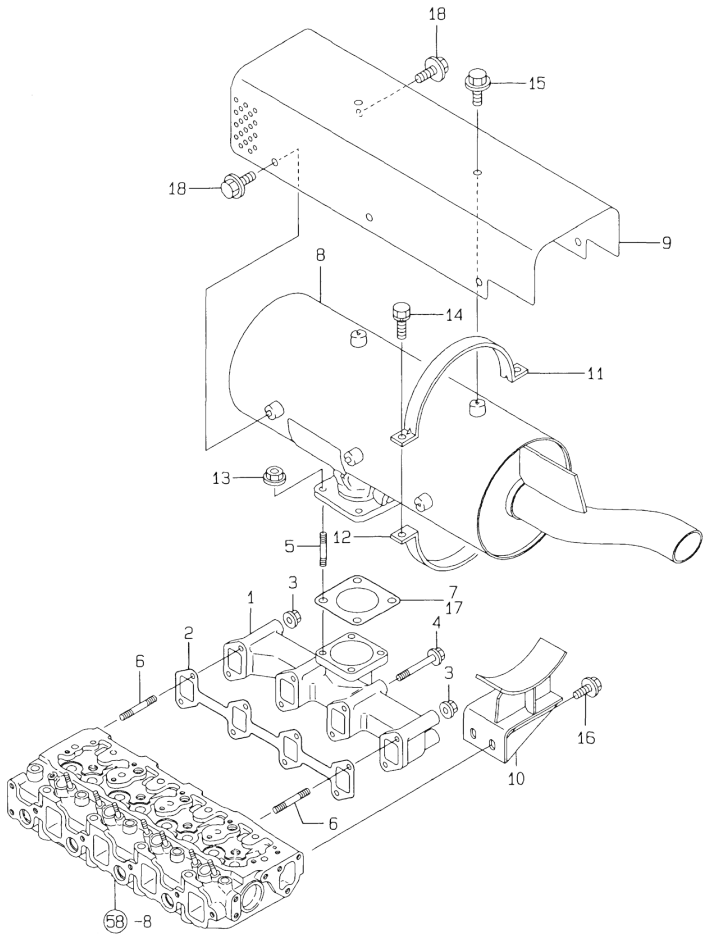
Fig.60. EXHAUST MANIFOLD & SILENCER
