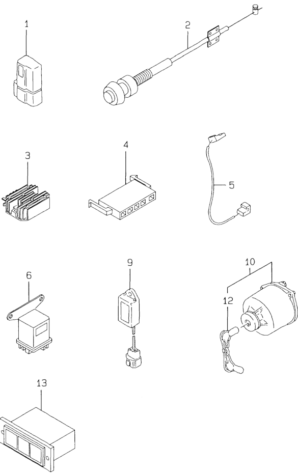
Fig.53. ELECTRICAL PARTS
