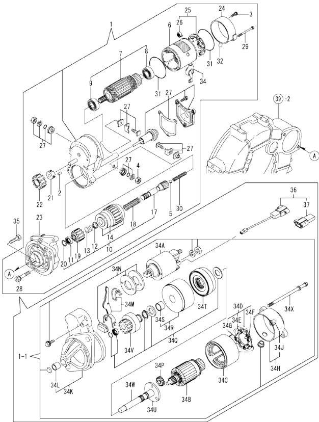
Fig.51. STARTING MOTOR
