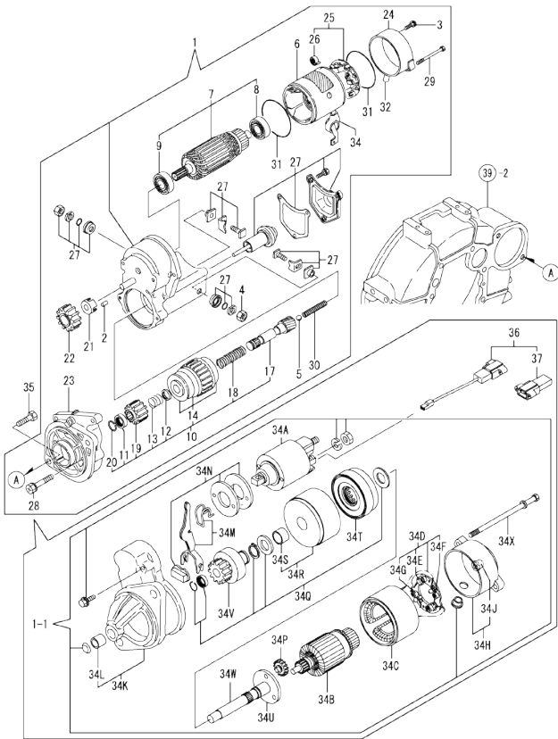
Fig.51. STARTING MOTOR
