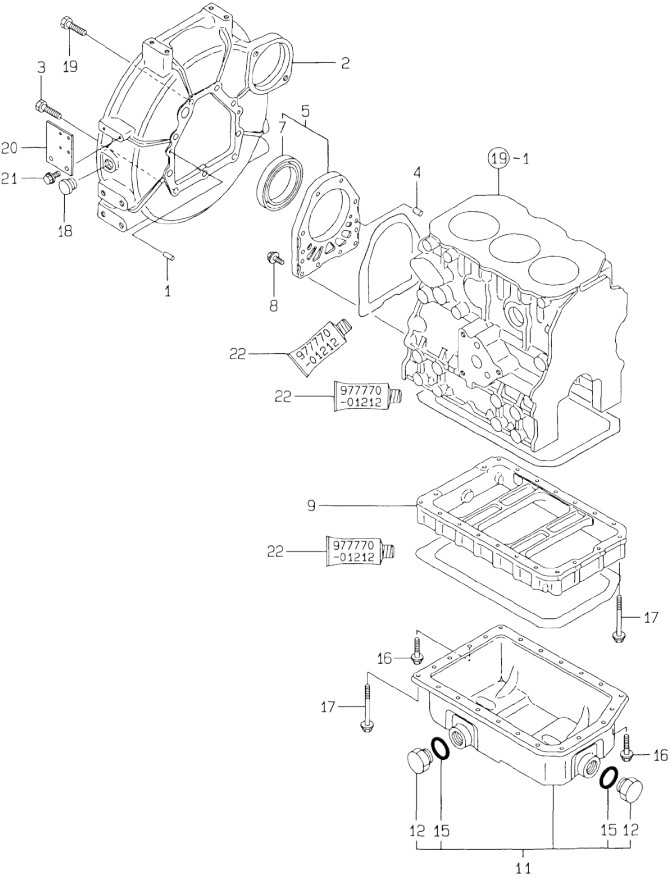
Fig.21. FLYWHEEL HOUSING & OIL SUMP
