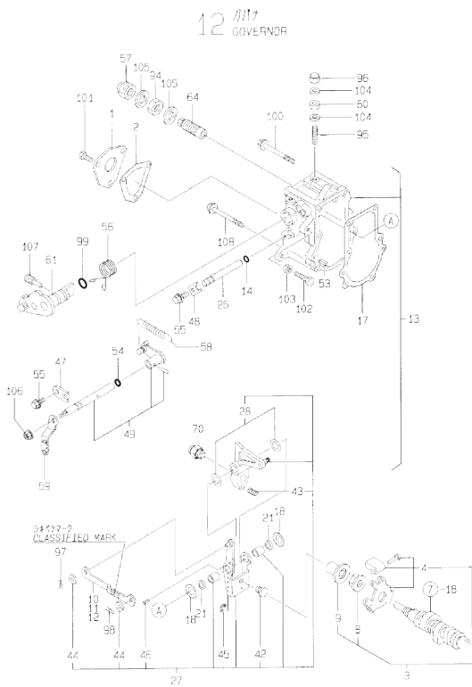
Fig.12. GOVERNOR
