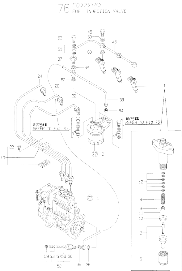
OCE10-M26900 ENGINE SECTION Fig.76. FUEL INJECTION VALVE
