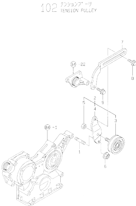
OCE10-M26900 ENGINE SECTION Fig.102. TENSION PULLEY
