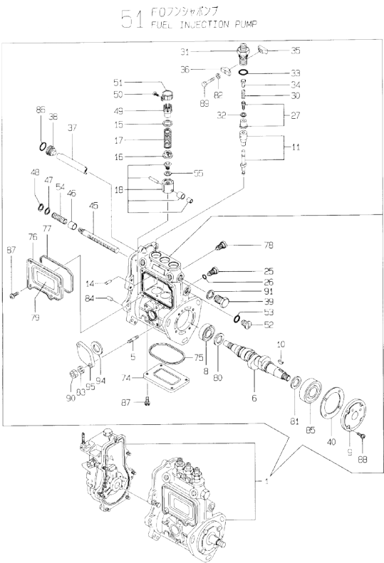
OCE10-M26900 ENGINE SECTION Fig.51. FUEL INJECTION PUMP
