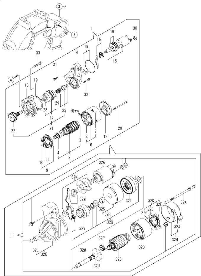
Fig.17. STARTING MOTOR
