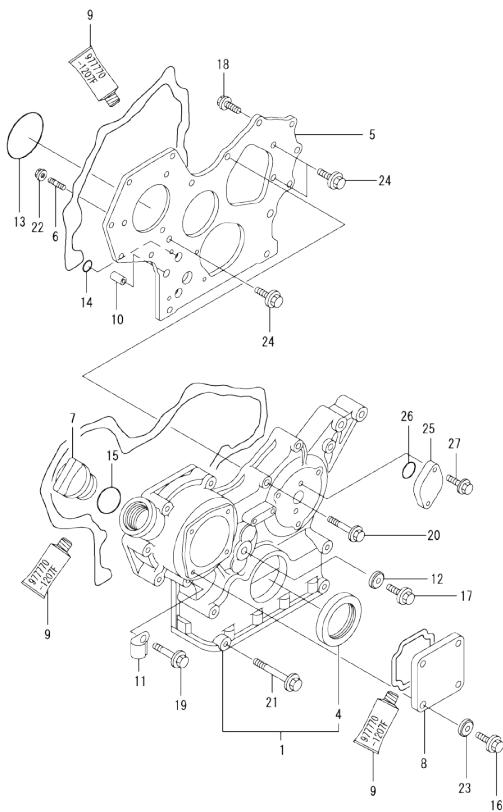
OCD10-M74101 ENGINE SECTION Fig.2. GEAR HOUSING
