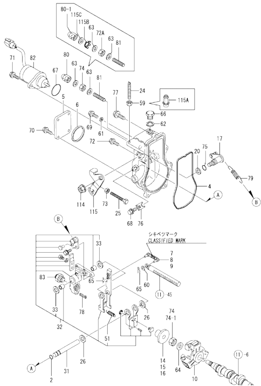
Fig.12. GOVERNOR
