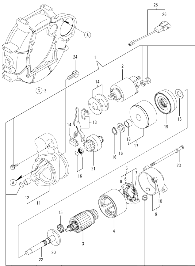
OCD10-M74101 ENGINE SECTION Fig.15. STARTING MOTOR
