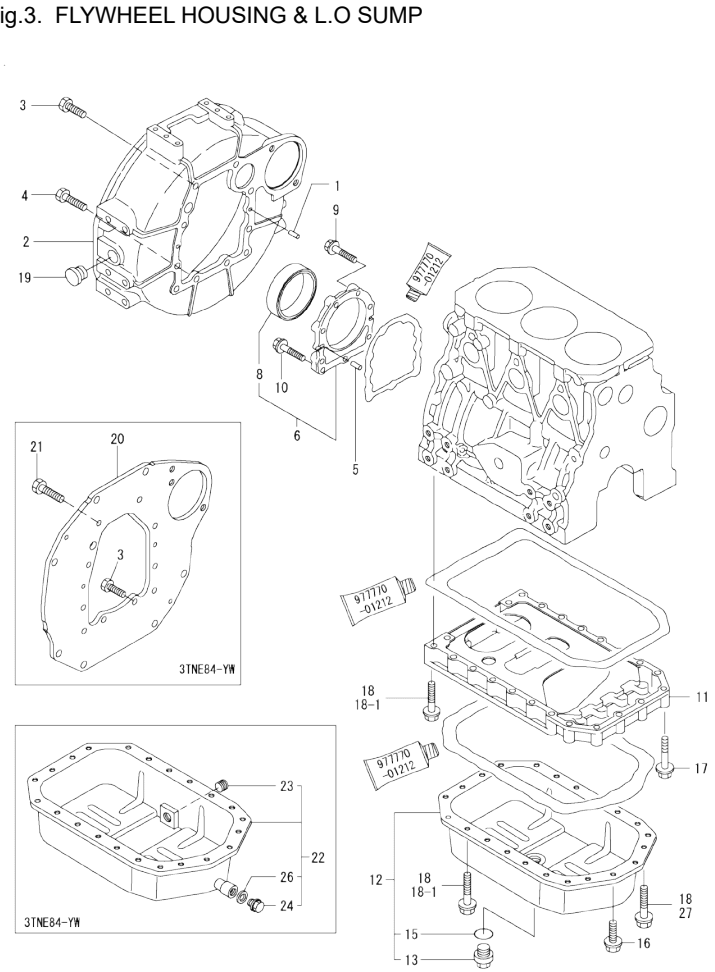
Fig.3. FLYWHEEL HOUSING & L.O SUMP
