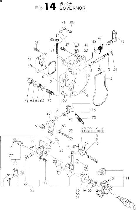
Fig.14. GOVERNOR
