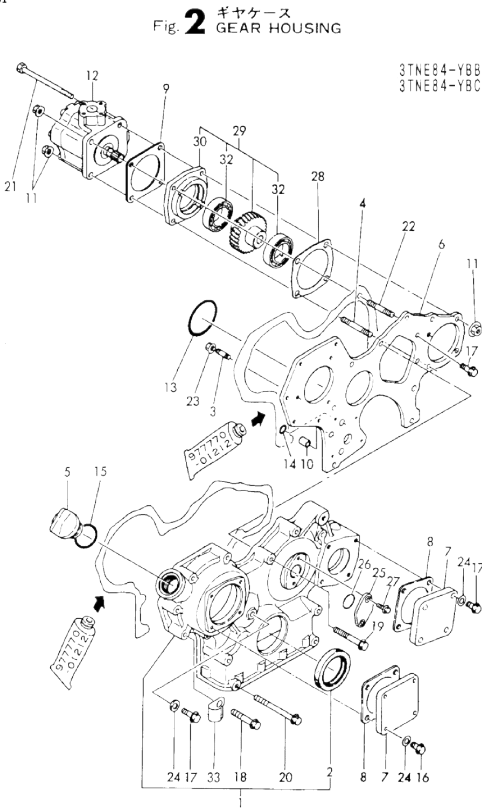
Fig.2. GEAR HOUSING
