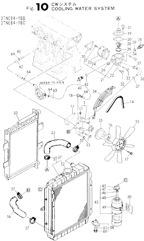
Fig.10. COOLING WATER SYSTEM
