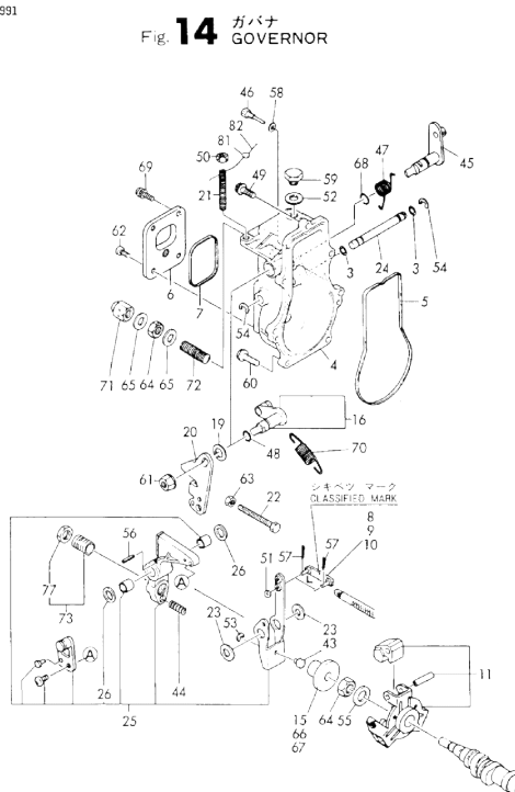
Fig.14. GOVERNOR
