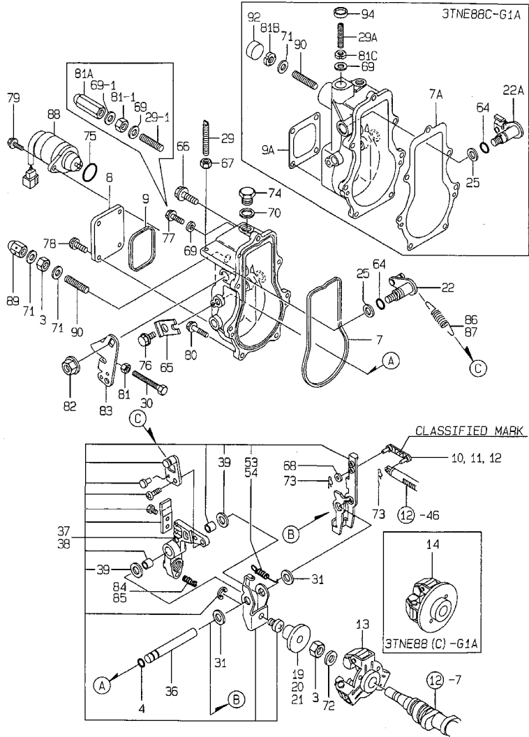
Fig.13. GOVERNOR
