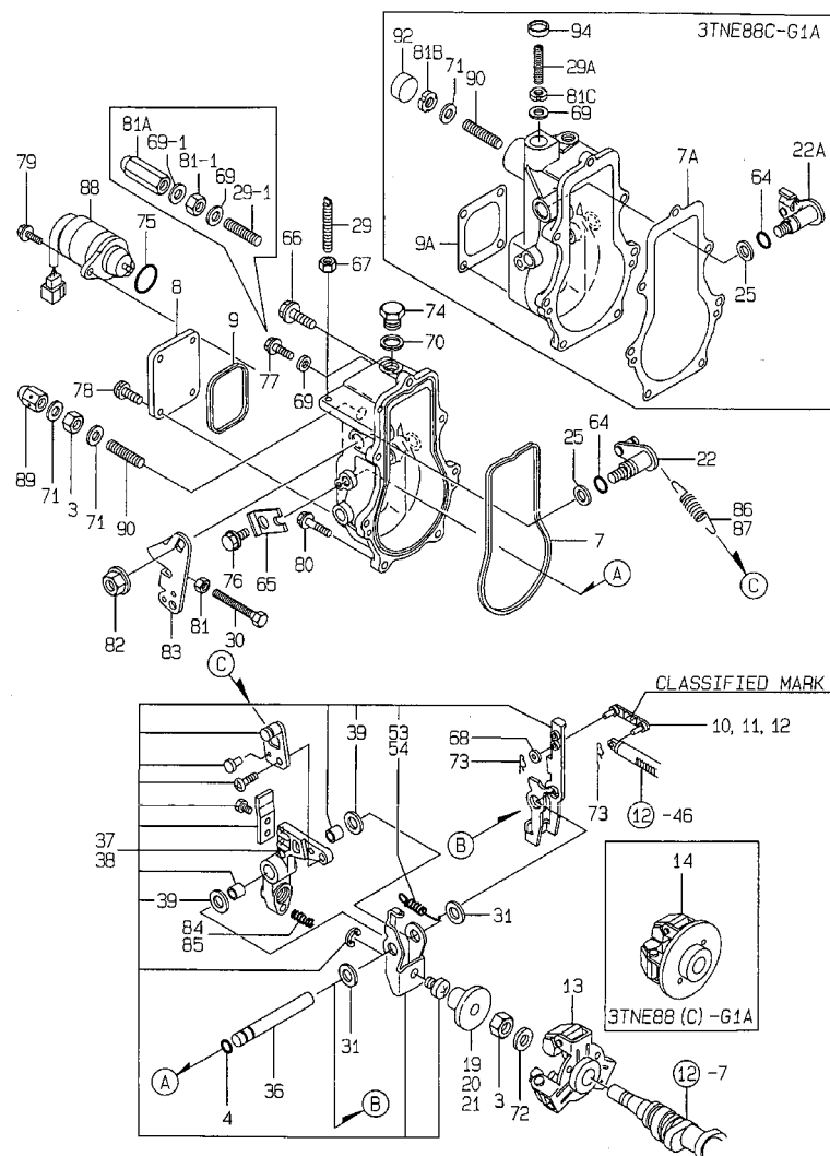
Fig.13. GOVERNOR
