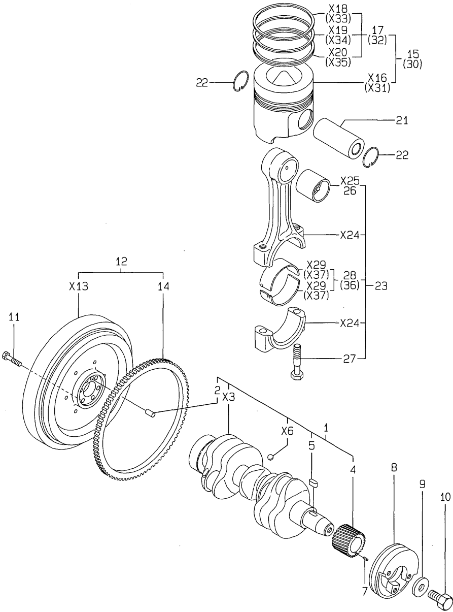
Fig.8. CRANKSHAFT & PISTON
