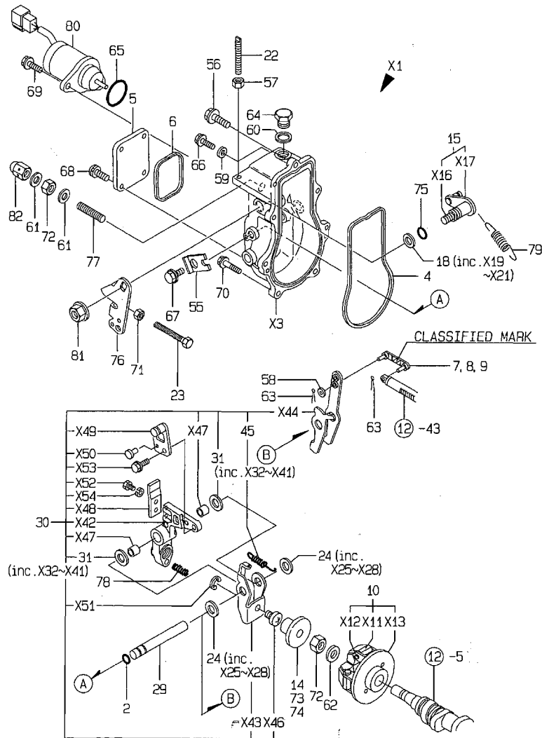
Fig.13. GOVERNOR
