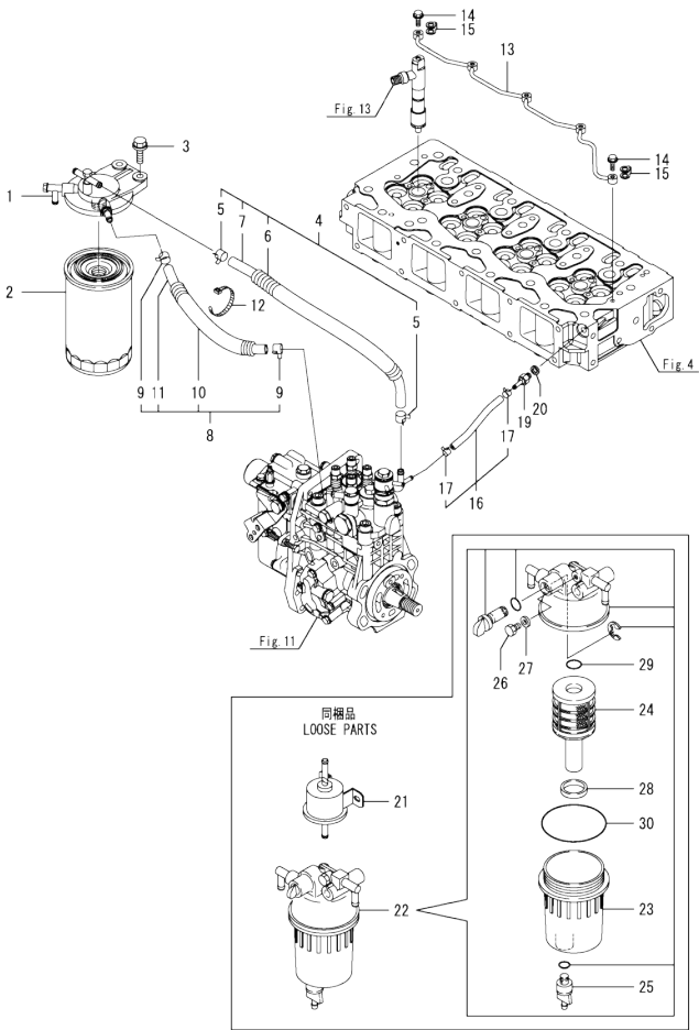
Fig.14. FUEL PIPE
