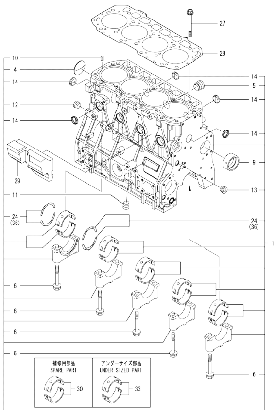
OCD50-M01730 4TNV94L-BVFN Fig.1. CYLINDER BLOCK
