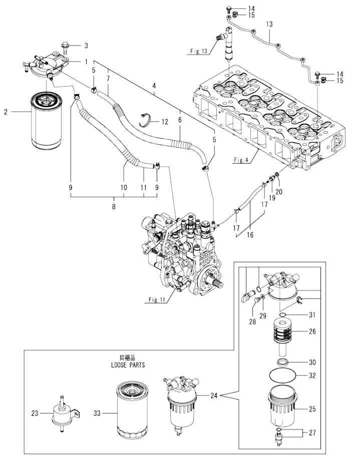
Fig.14. FUEL PIPE
