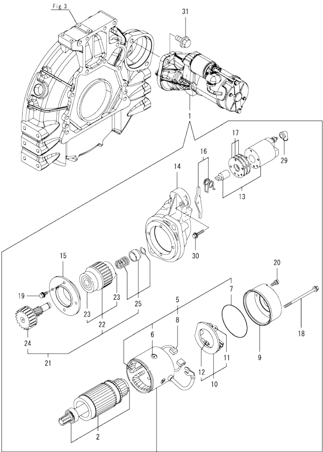
Fig.15. STARTER MOTOR
