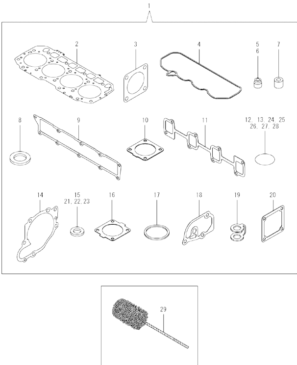
Fig.17. GASKET SET
