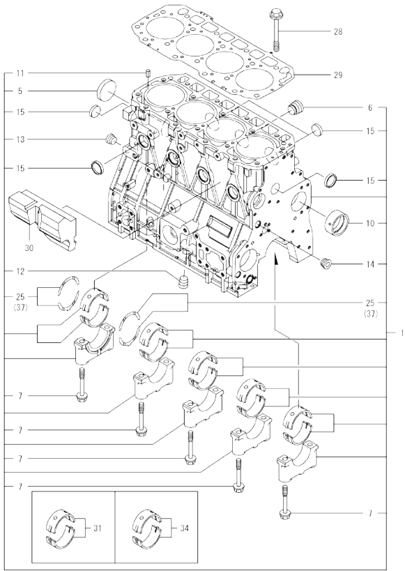
0CD50-M00060 4TNV94L-BVSU Fig.1. CYLINDER BLOCK
