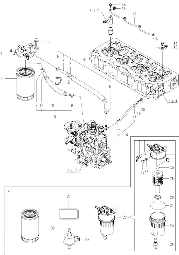
Fig.14. FUEL PIPE
