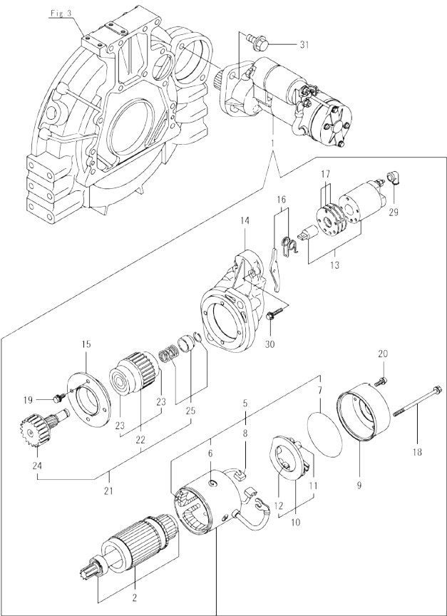
OCD50-M00060 4TNV94L-BVSU Fig.15. STARTER MOTOR
