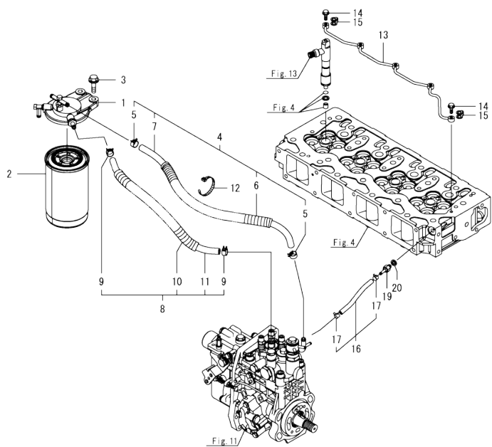
OCD50-M05590 ENGINE Fig.14. FUEL PIPE
