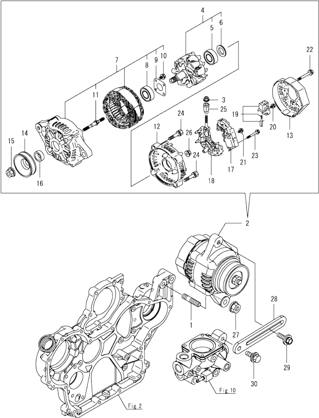
OCD50-M03630 ENGINE Fig.16. GENERATOR
