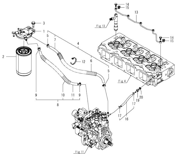
OCD50-M02480 ENGINE Fig.14. FUEL PIPE
