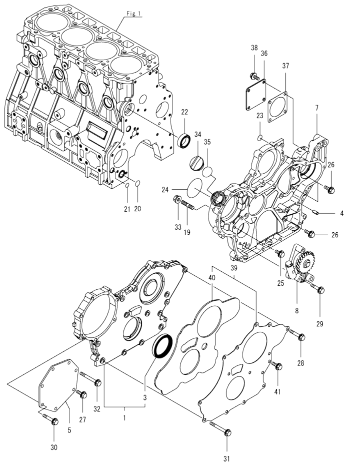
Fig.2. GEAR HOUSING
