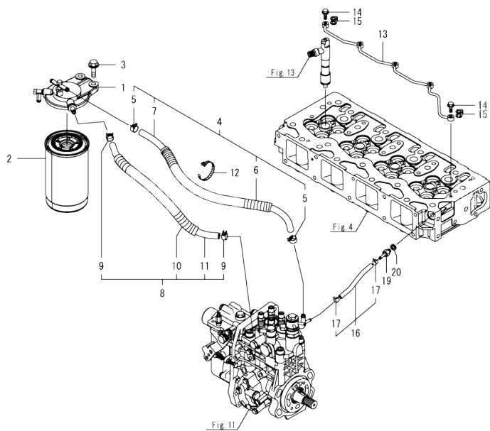
OCD50-M02650 ENGINE Fig.14. FUEL PIPE
