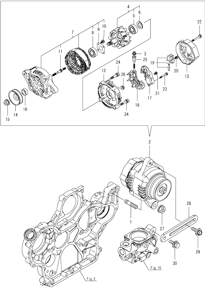
OCD50-M02650 ENGINE Fig.16. GENERATOR
