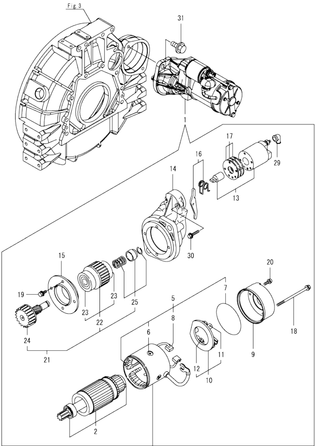
Fig.15. STARTER MOTOR
