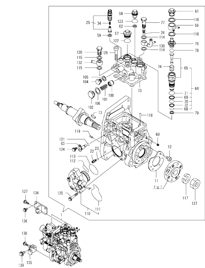
Fig.11. FUEL INJECTION PUMP
