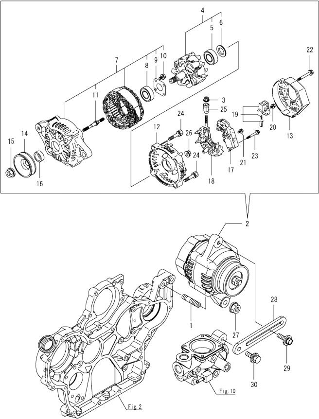
OCD50-M03690 ENGINE Fig.16. GENERATOR
