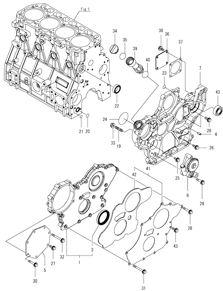
Fig.2. GEAR HOUSING
