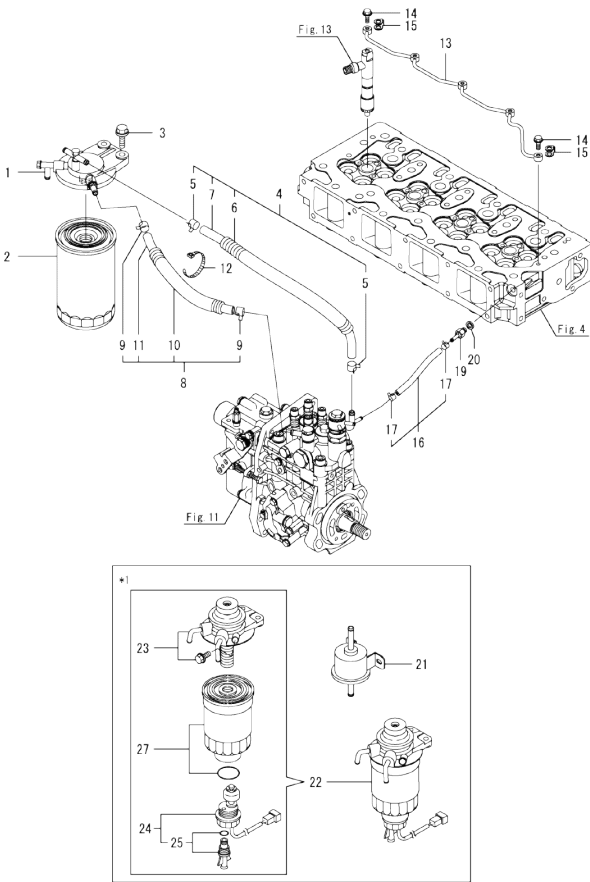
Fig.14. FUEL PIPE
