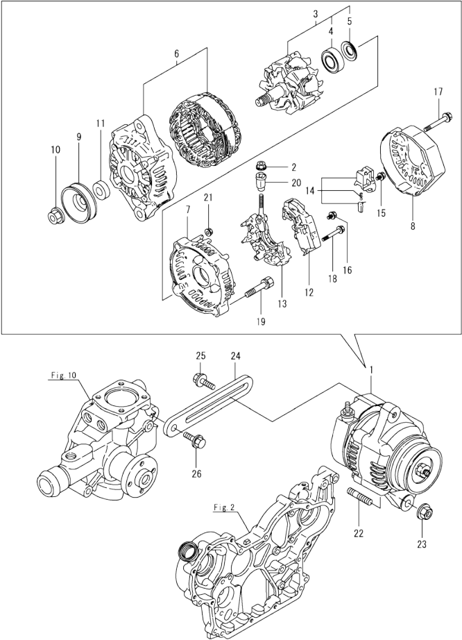
OCD50-M02600 ENGINE Fig.16. GENERATOR
