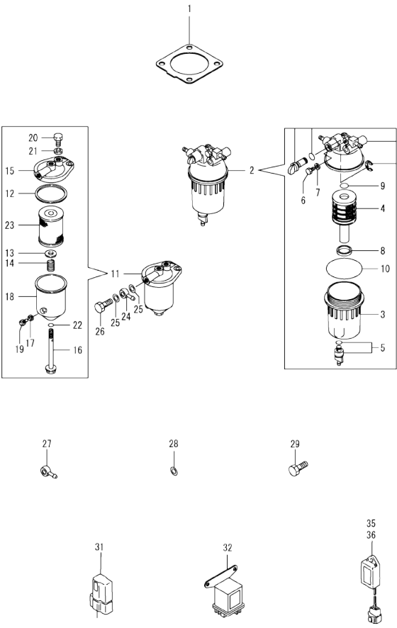
Fig.17. ACCESSORY
