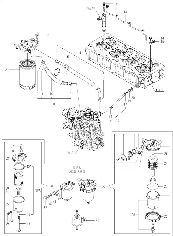
0CW10-M72500 ENGINE Fig.14. FUEL PIPE
