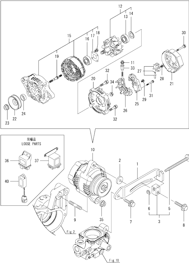
0CW10-M72500 ENGINE Fig.16. GENERATOR
